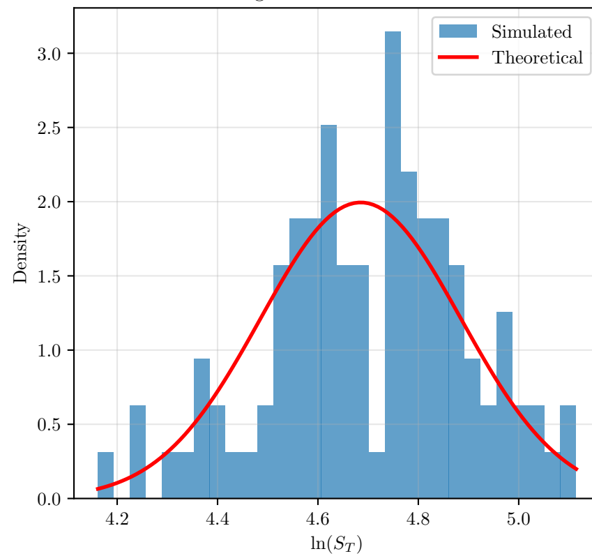
Euler-Maruyama Convergence
