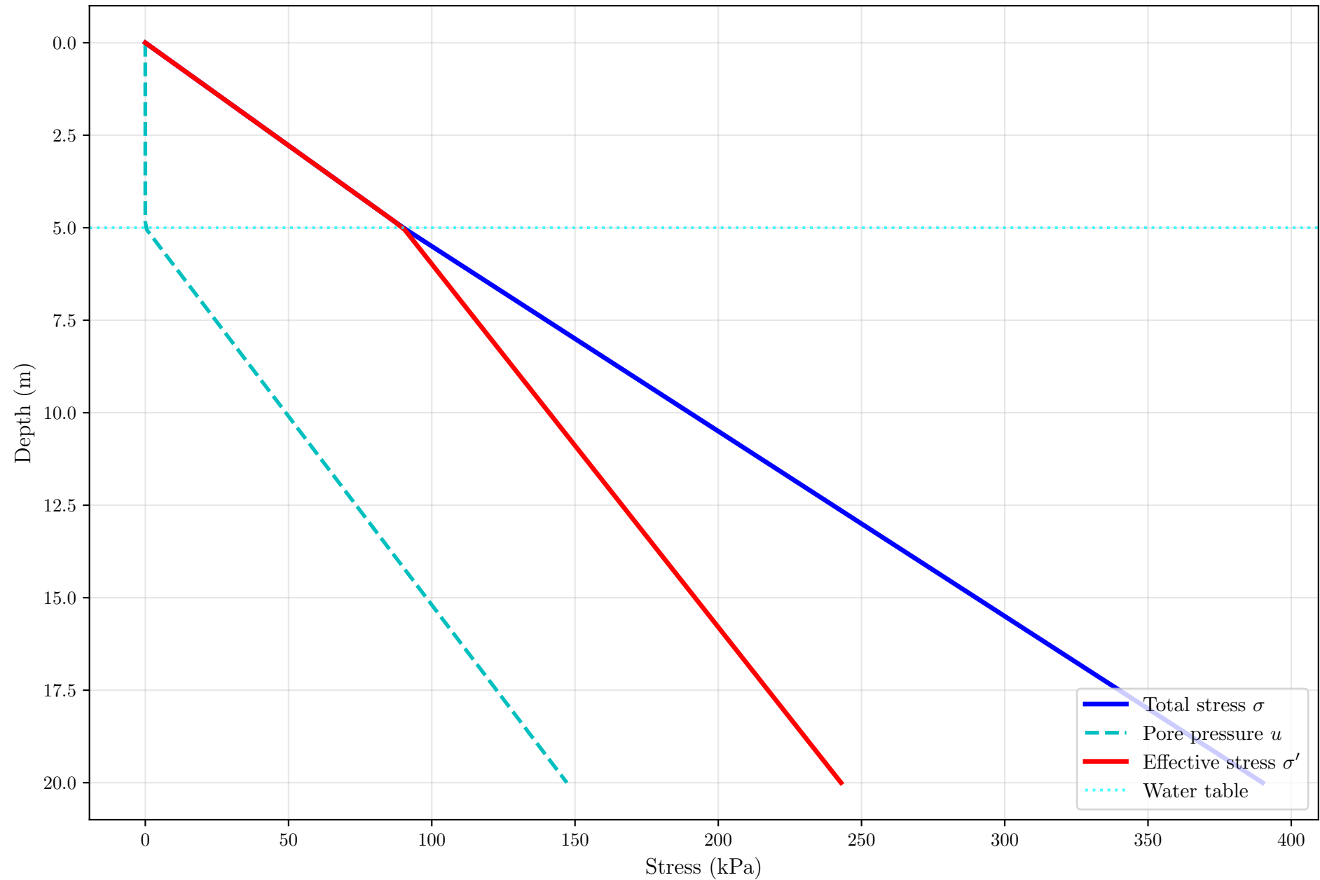
Effective Stress Profile with Water Table at 5 m Depth
