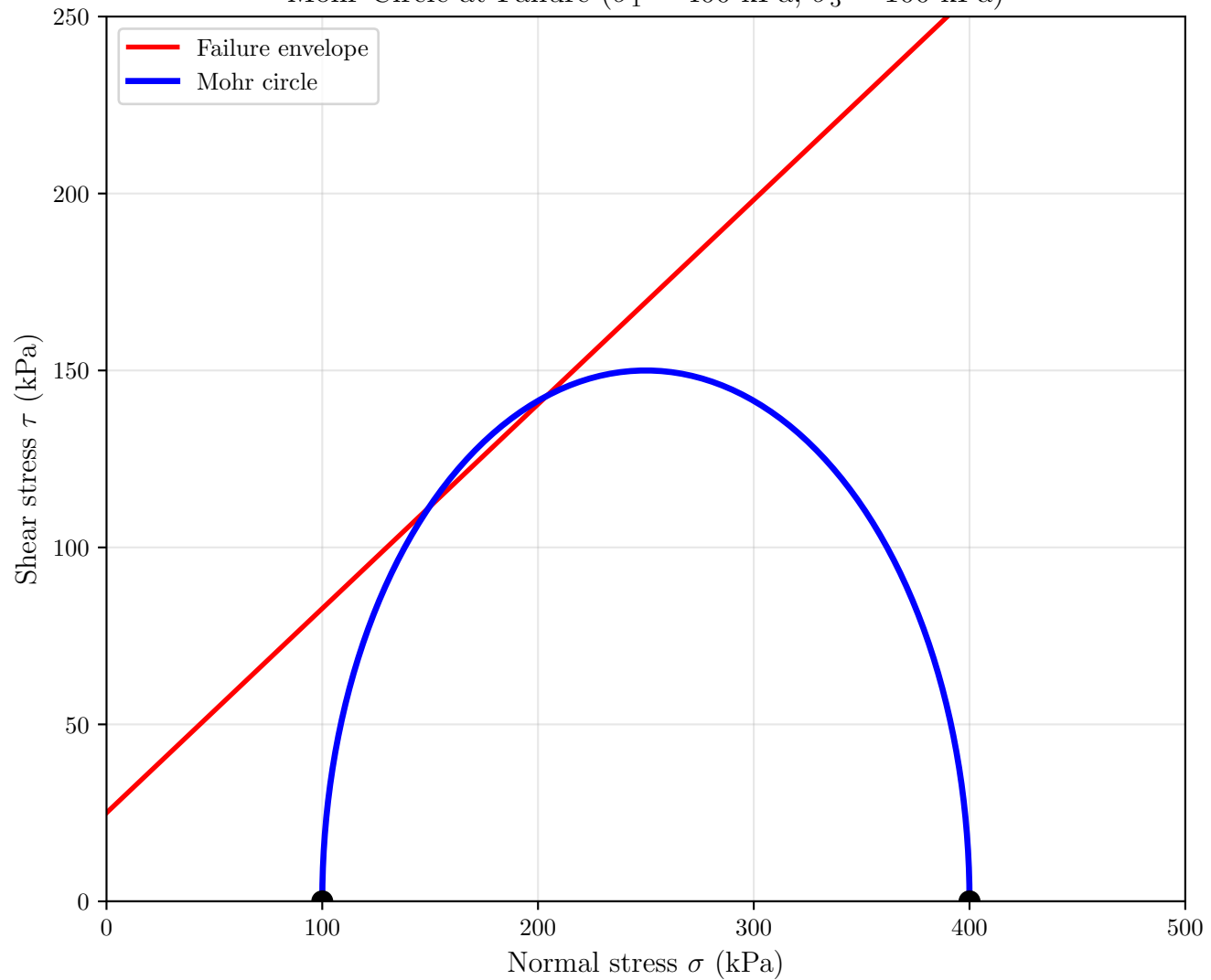
Mohr Circle at Failure ( \sigma_1 = 400 kPa, \sigma_3 = 100 kPa)
