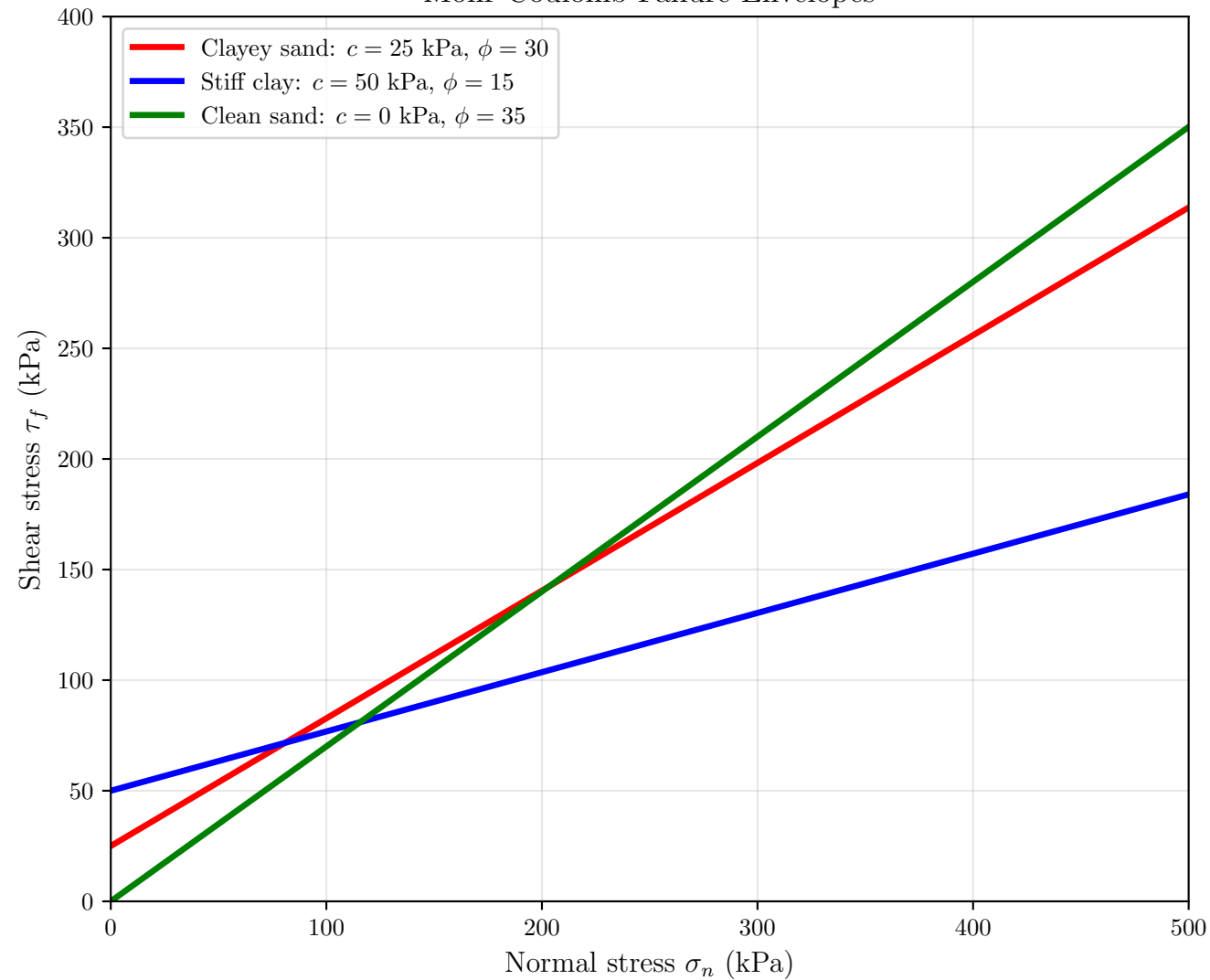
Mohr-Coulomb Failure Envelopes
