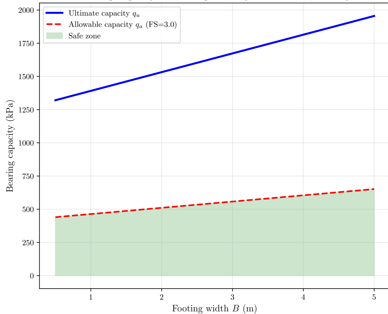
Bearing Capacity vs. Footing Width ( c = 25.0 kPa, \phi = 30.0 )
