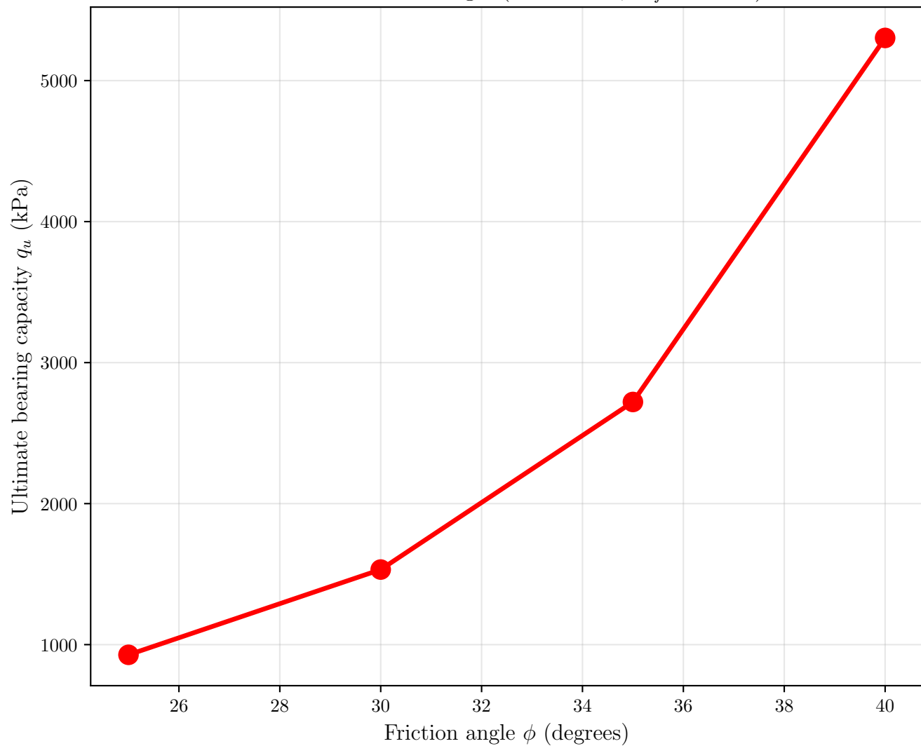
Effect of Friction Angle ( B = 2.0 m, D_f = 1.5 m)
