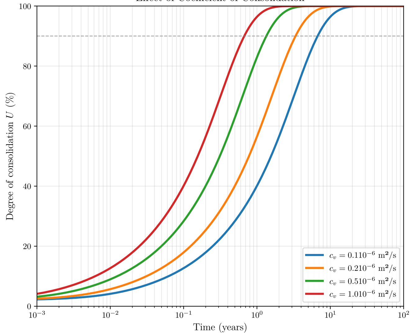
Effect of Coefficient of Consolidation
