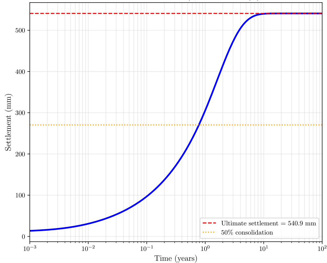
Consolidation Settlement ( c_v = 0.210^{-6} \text{ m}^2/\text{s} )
