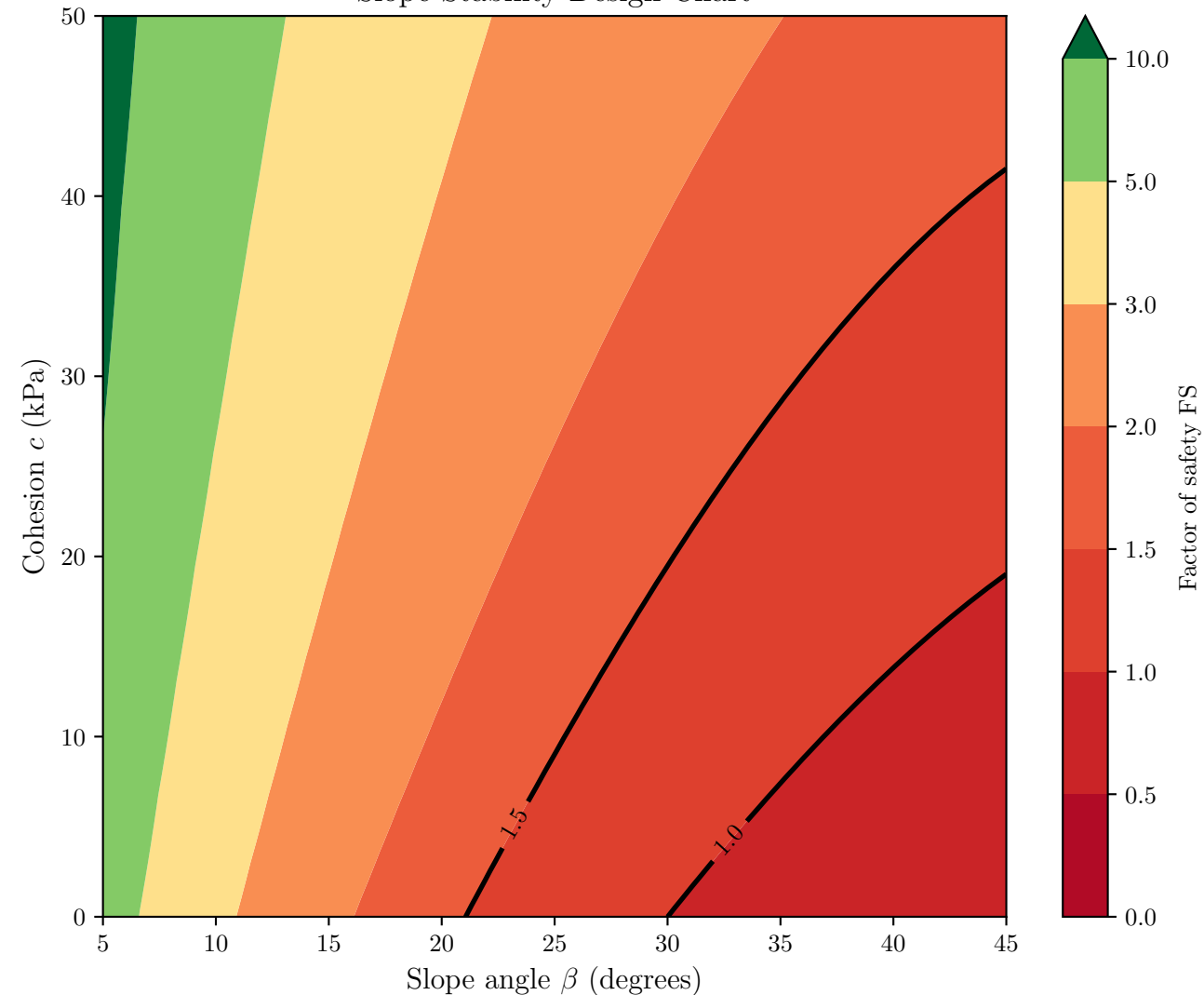
Slope Stability Design Chart
