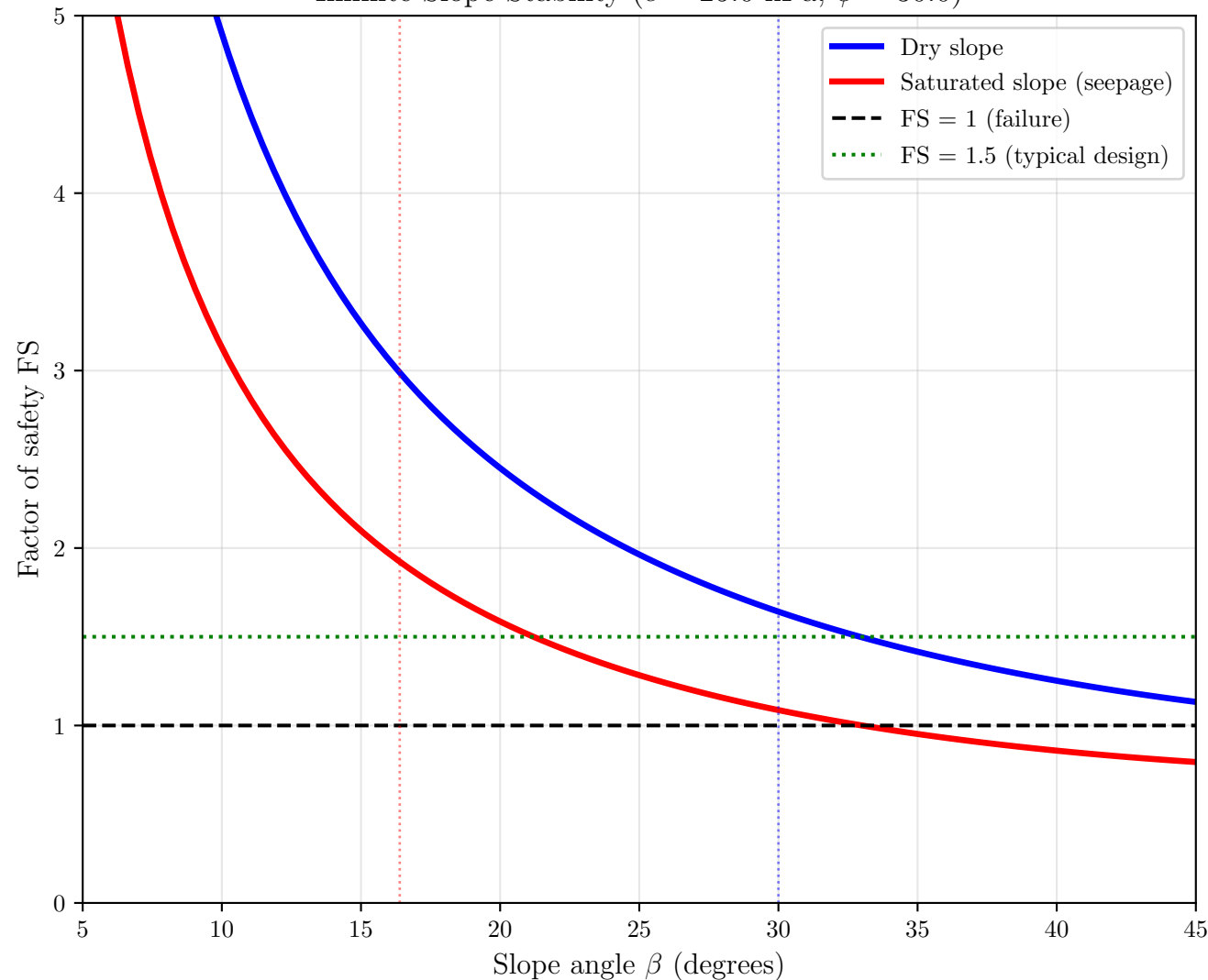
Infinite Slope Stability ( c = 25.0 kPa, \phi = 30.0 )
