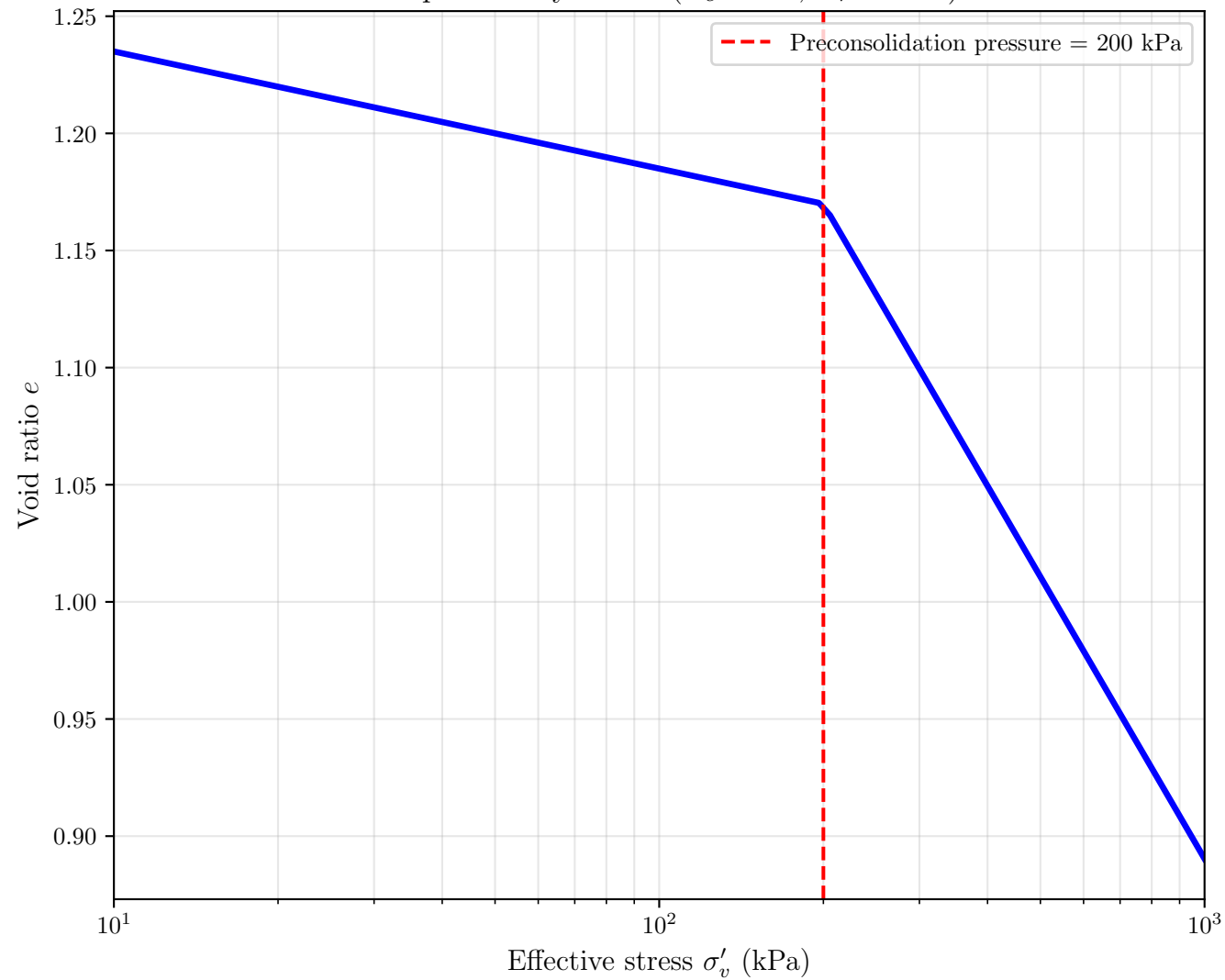
Compressibility Curve ( C_c = 0.4 , C_r = 0.05 )
