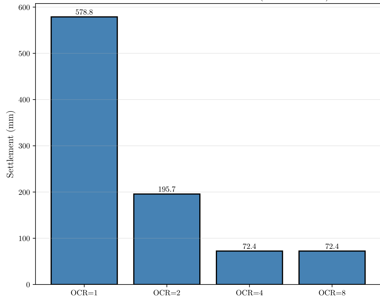
Settlement vs. Overconsolidation Ratio ( \Delta\sigma = 150 kPa)
