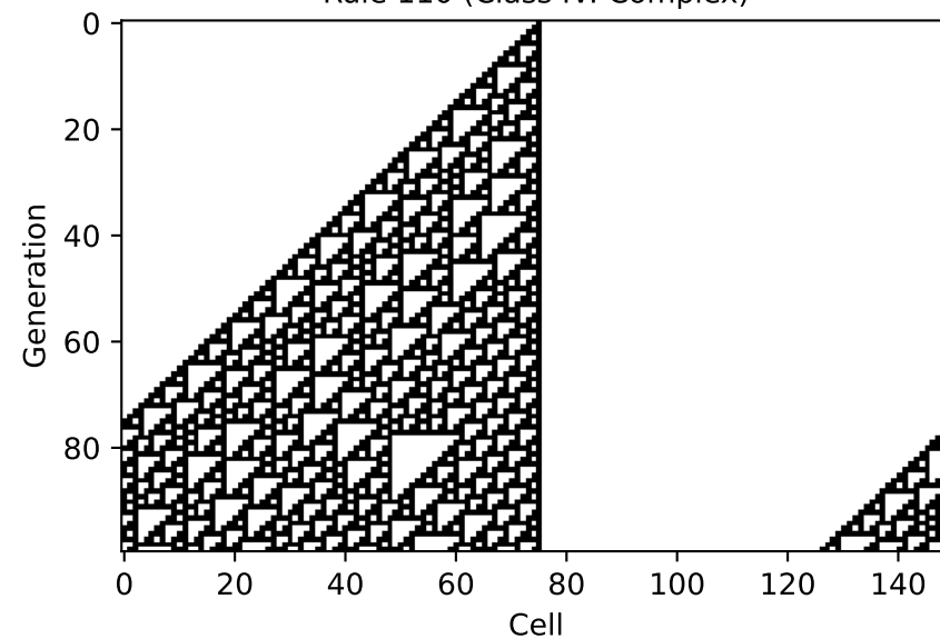
Rule 110 Density Evolution
