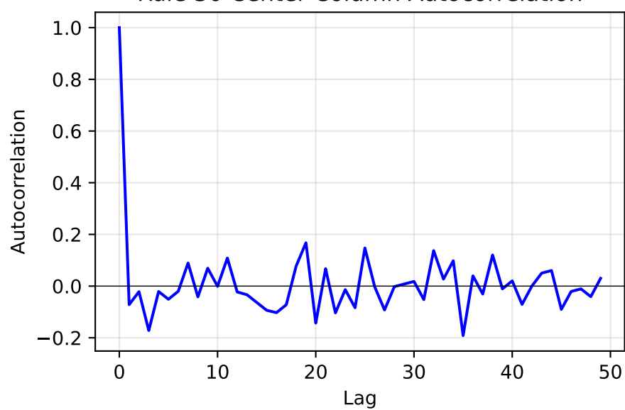
Rule 30 Center Column Autocorrelation
