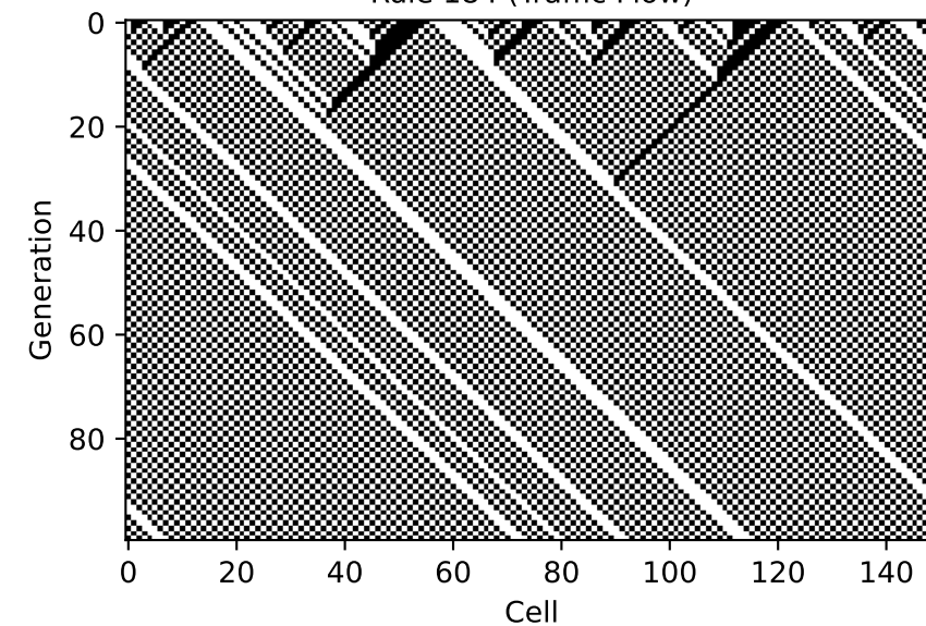
Rule 184 Density Evolution
