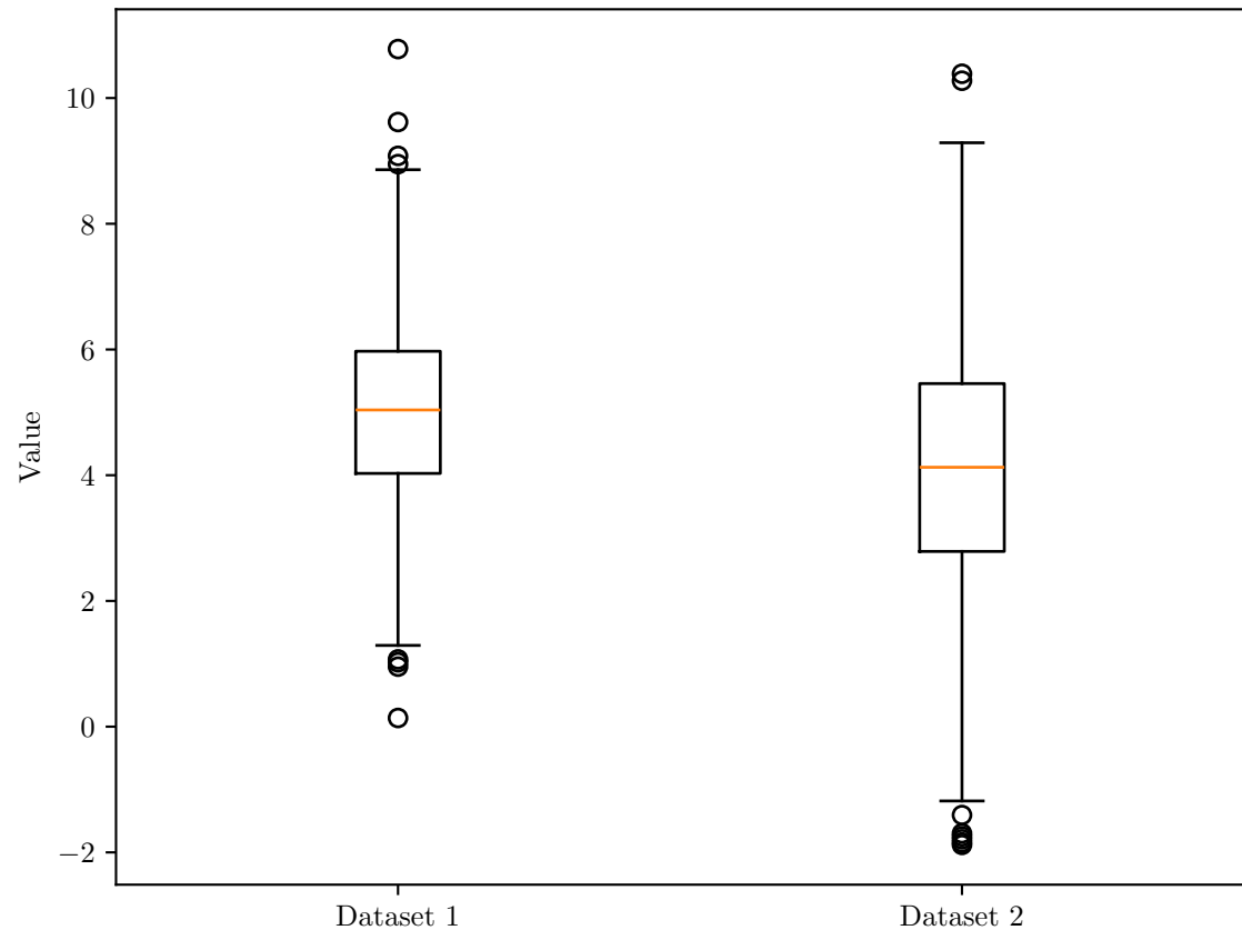
Box Plot
