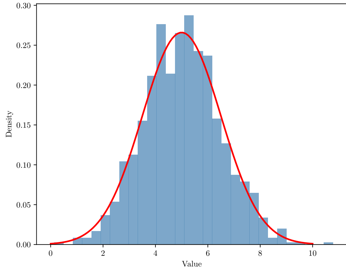
Distribution
