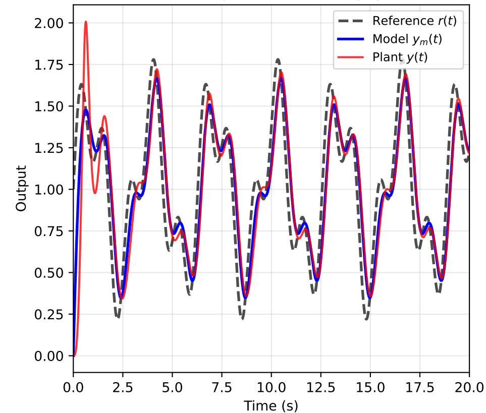
Feedforward Gain Adaptation
