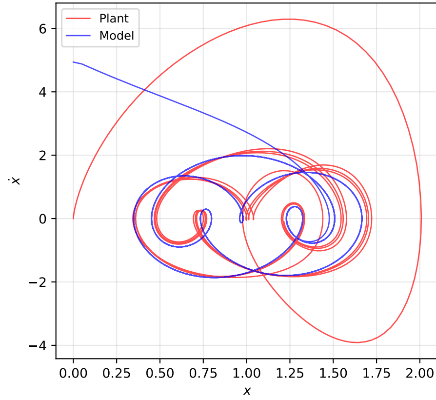
Phase Portrait
