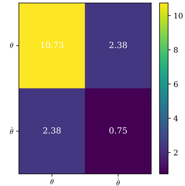
Riccati Matrix P
