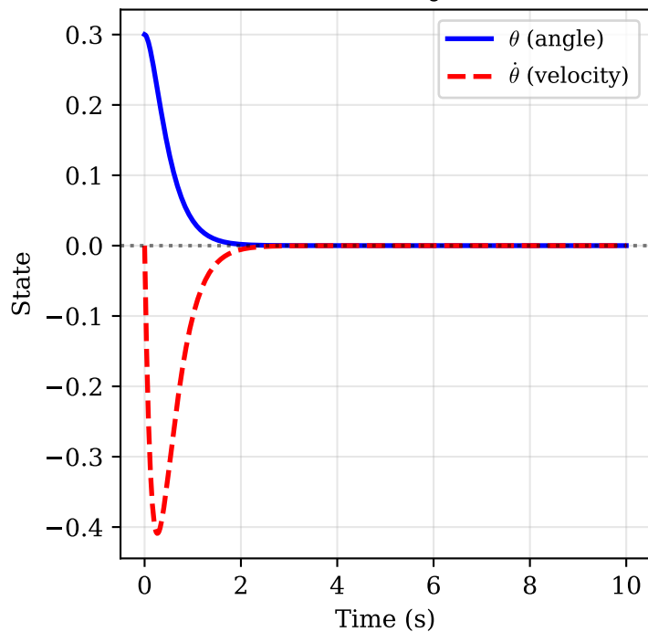
PMP: State Trajectories
