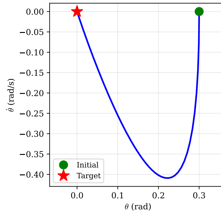
PMP: Optimal Control
