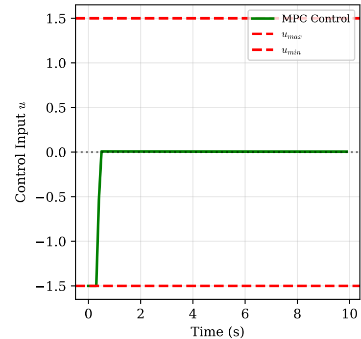
MPC: Constrained Control
