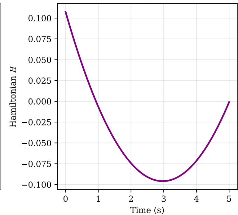
MPC: Constrained Control
