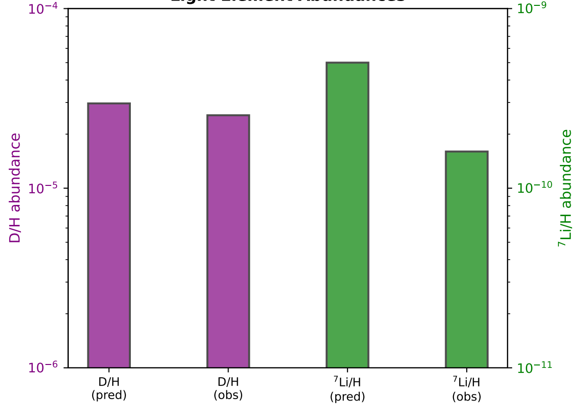
Light Element Abundances
