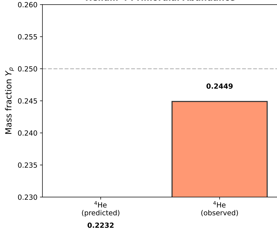
Helium-4 Primordial Abundance
