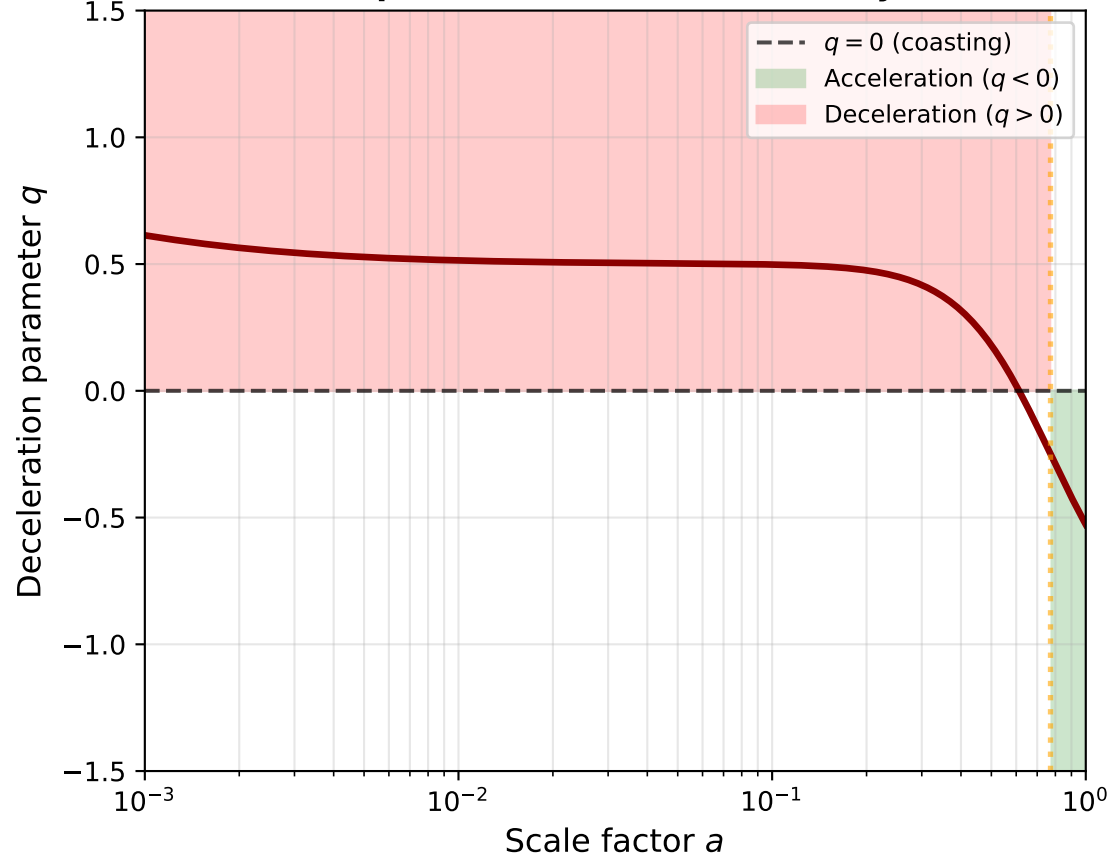
Expansion Acceleration History
