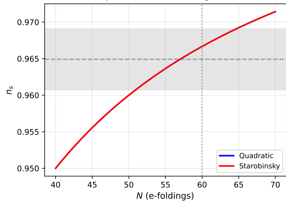
n_s Dependence on e-folding Number
