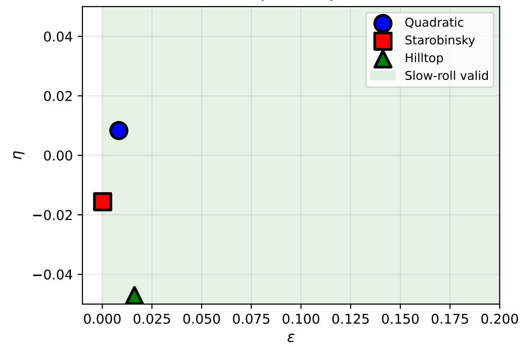
Phase Space: \epsilon - \eta Plane
