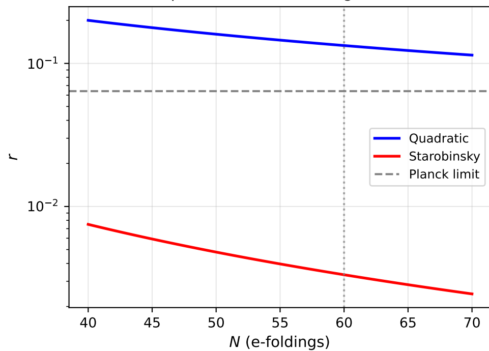
r Dependence on e-folding Number
