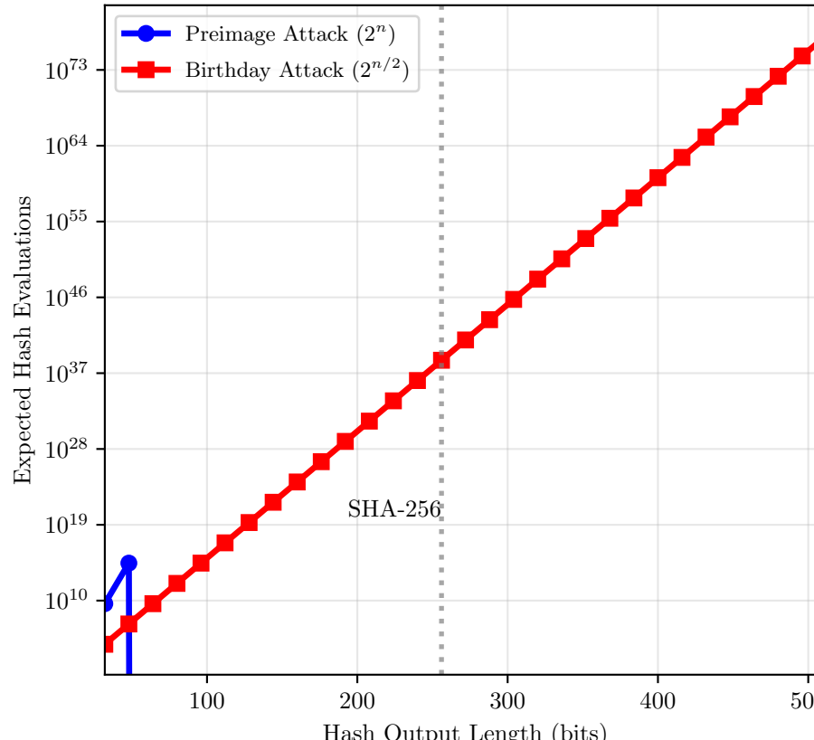
Birthday Bound: Required Hash Evaluations
