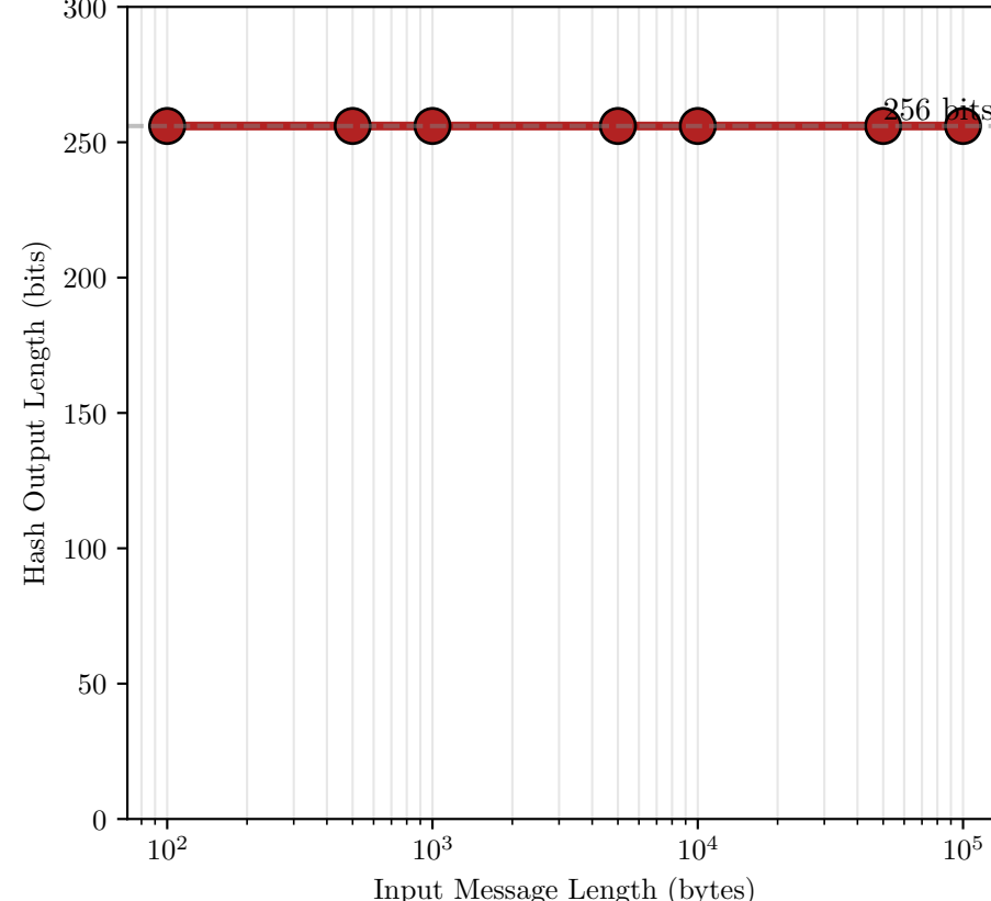
Fixed-Length Output Property
