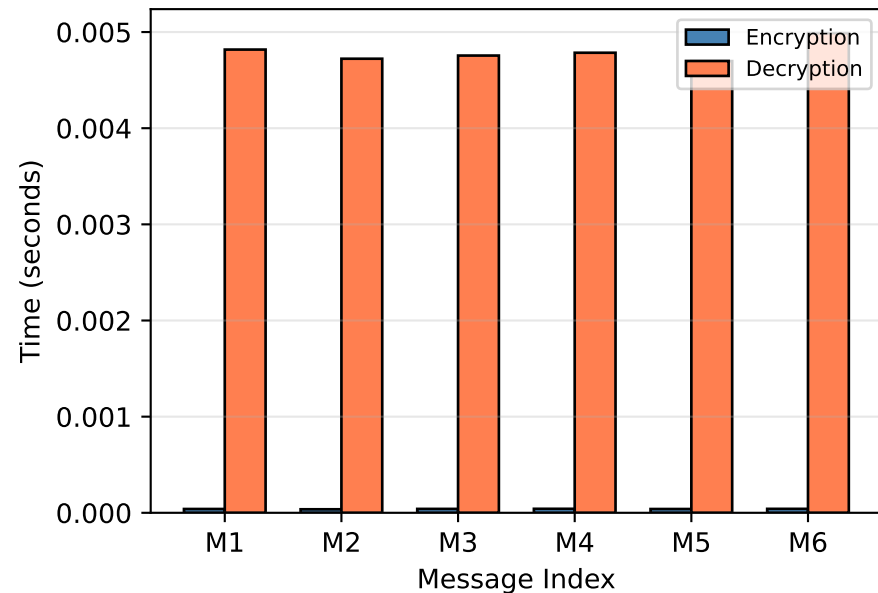
Cipher Operation Performance (1024-bit)
