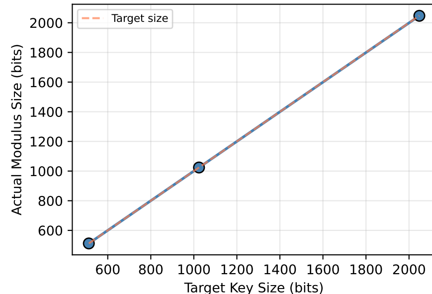
Key Size Validation
