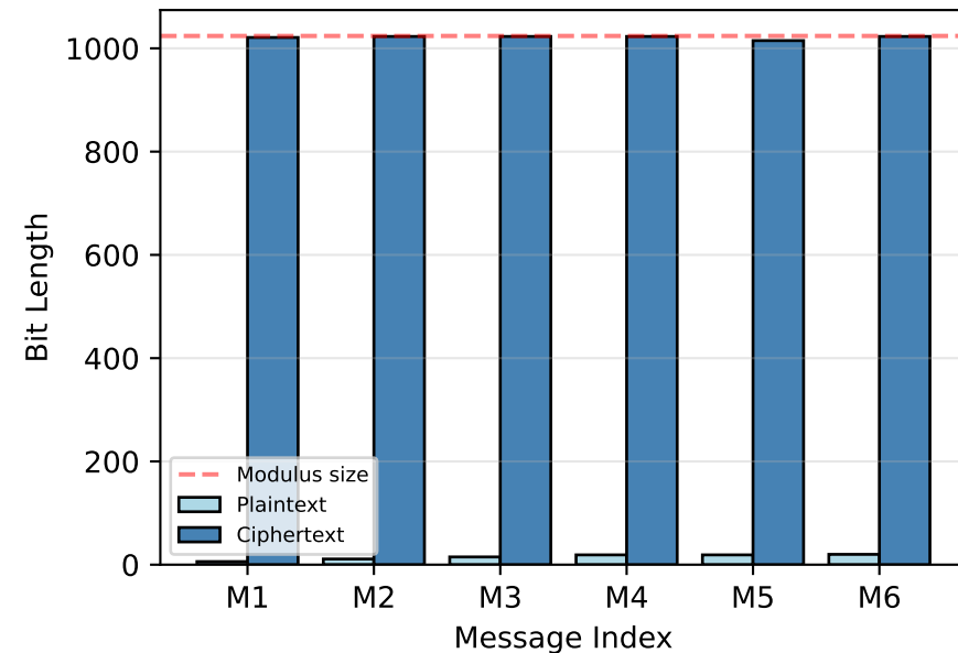
Message Expansion (Plaintext → Ciphertext)
