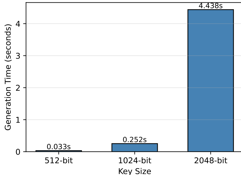
Key Generation Performance
