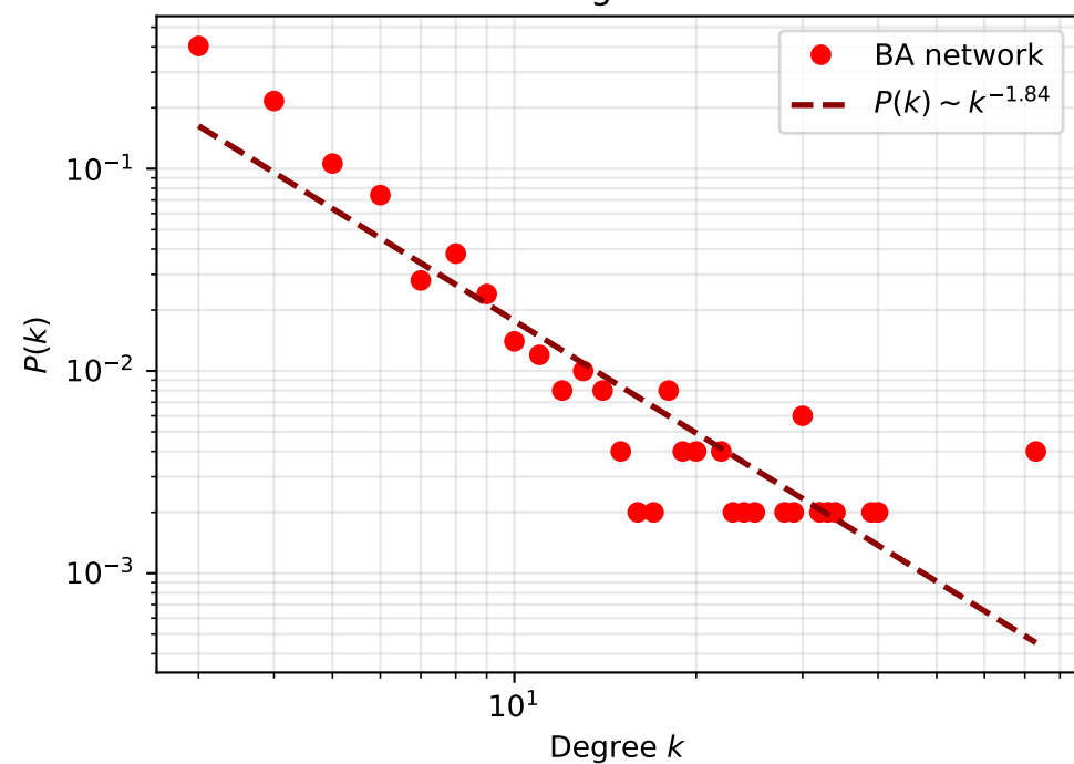
Scale-Free Degree Distribution
