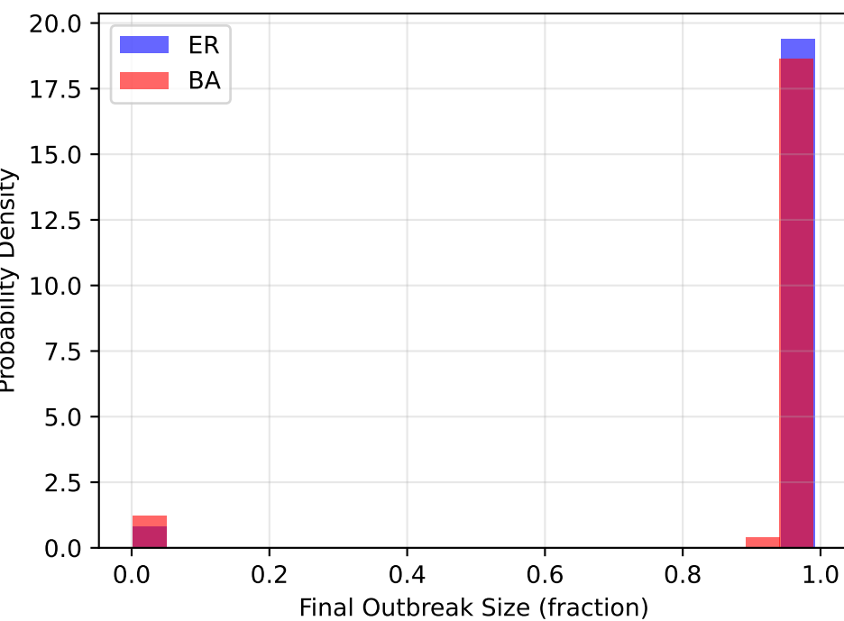
Outbreak Size Distribution
