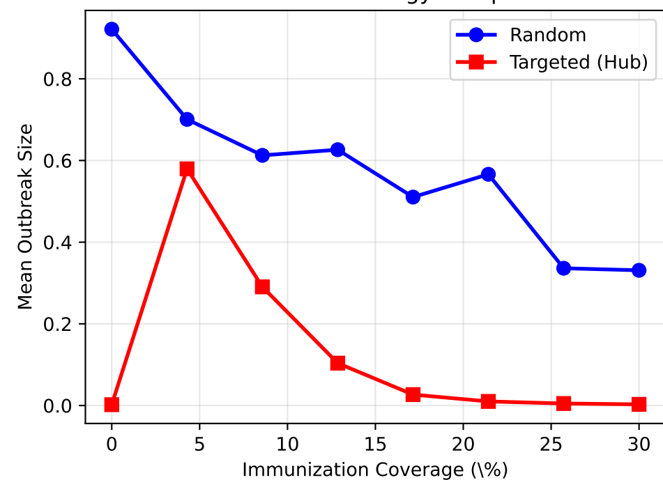
Immunization Strategy Comparison
