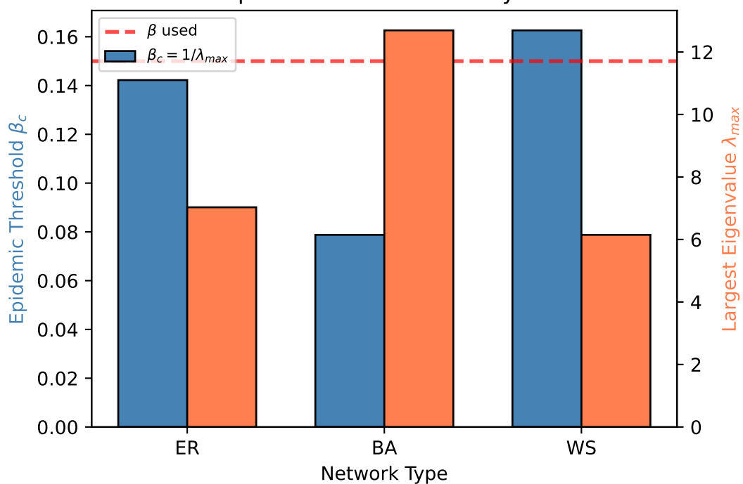
Epidemic Threshold Analysis
