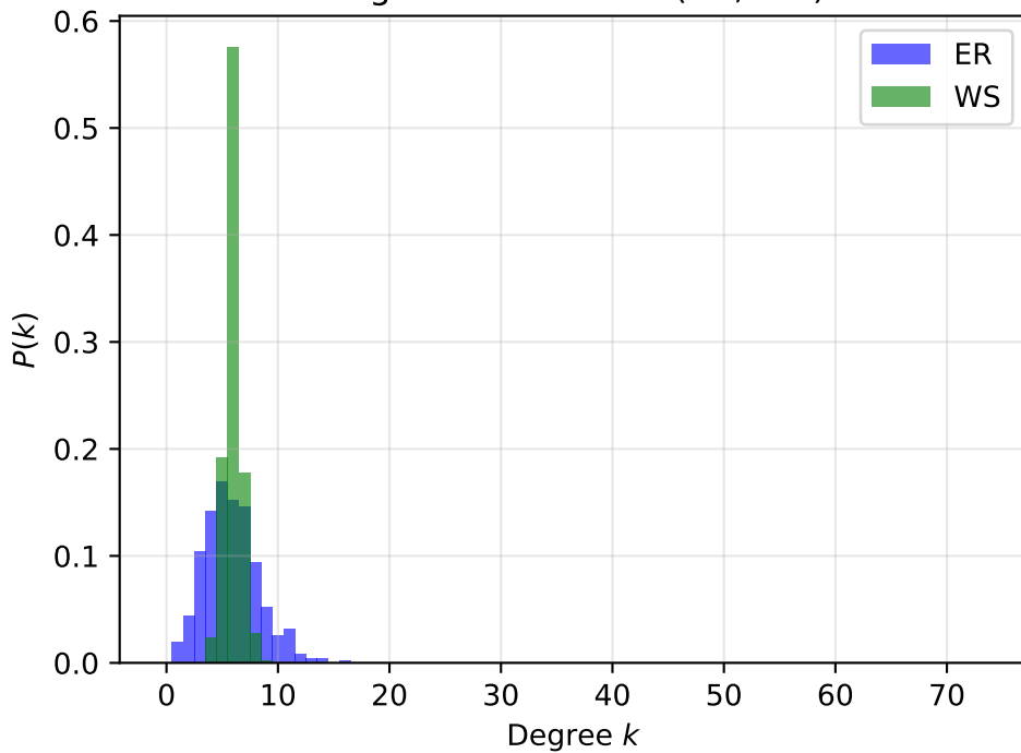
Degree Distribution (ER, WS)
