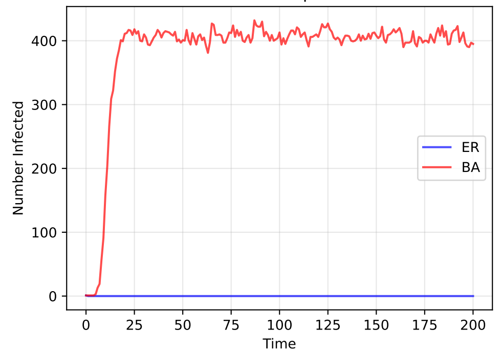
SIS Endemic Equilibrium
