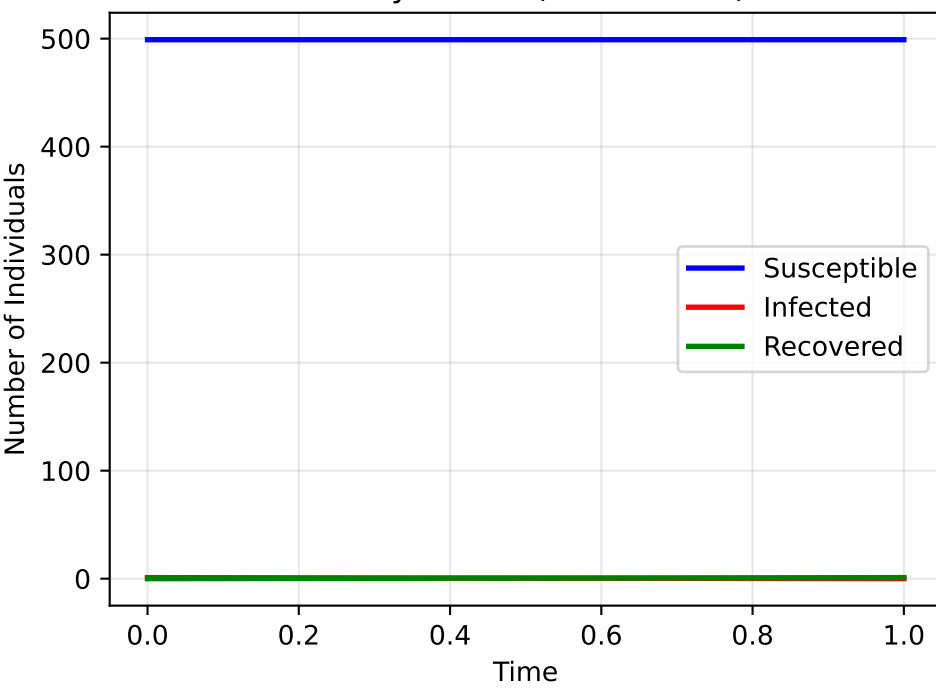
SIR Dynamics (BA Network)
