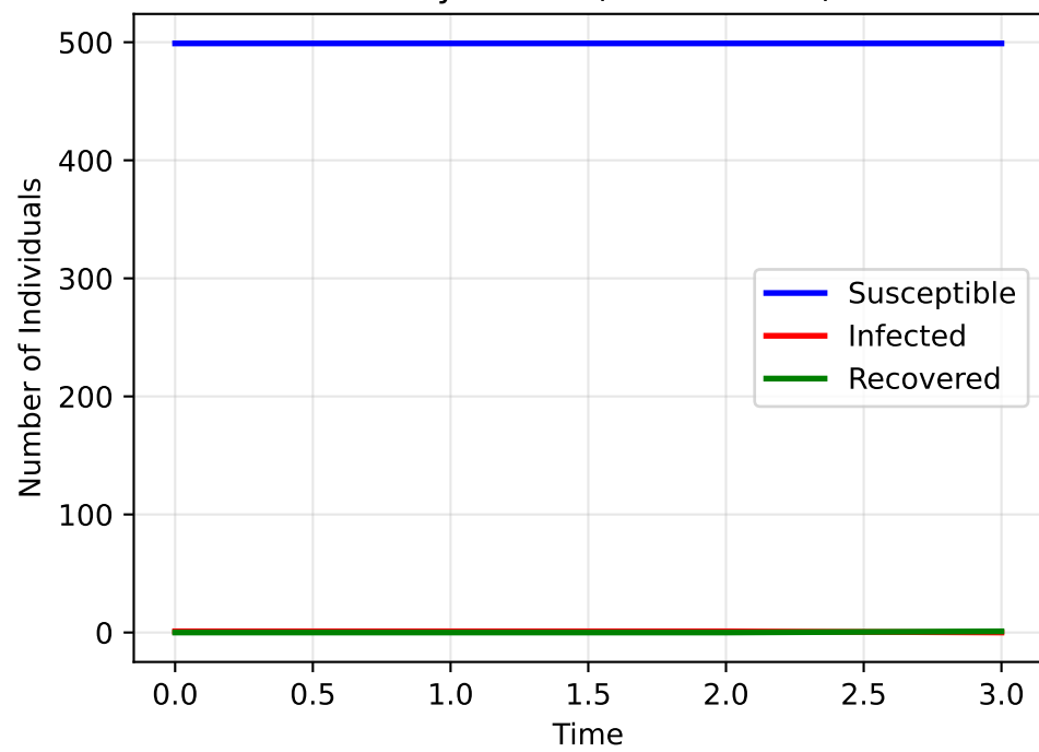
SIR Dynamics (WS Network)
