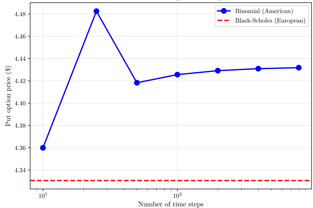
Binomial Tree Convergence: Put Option
