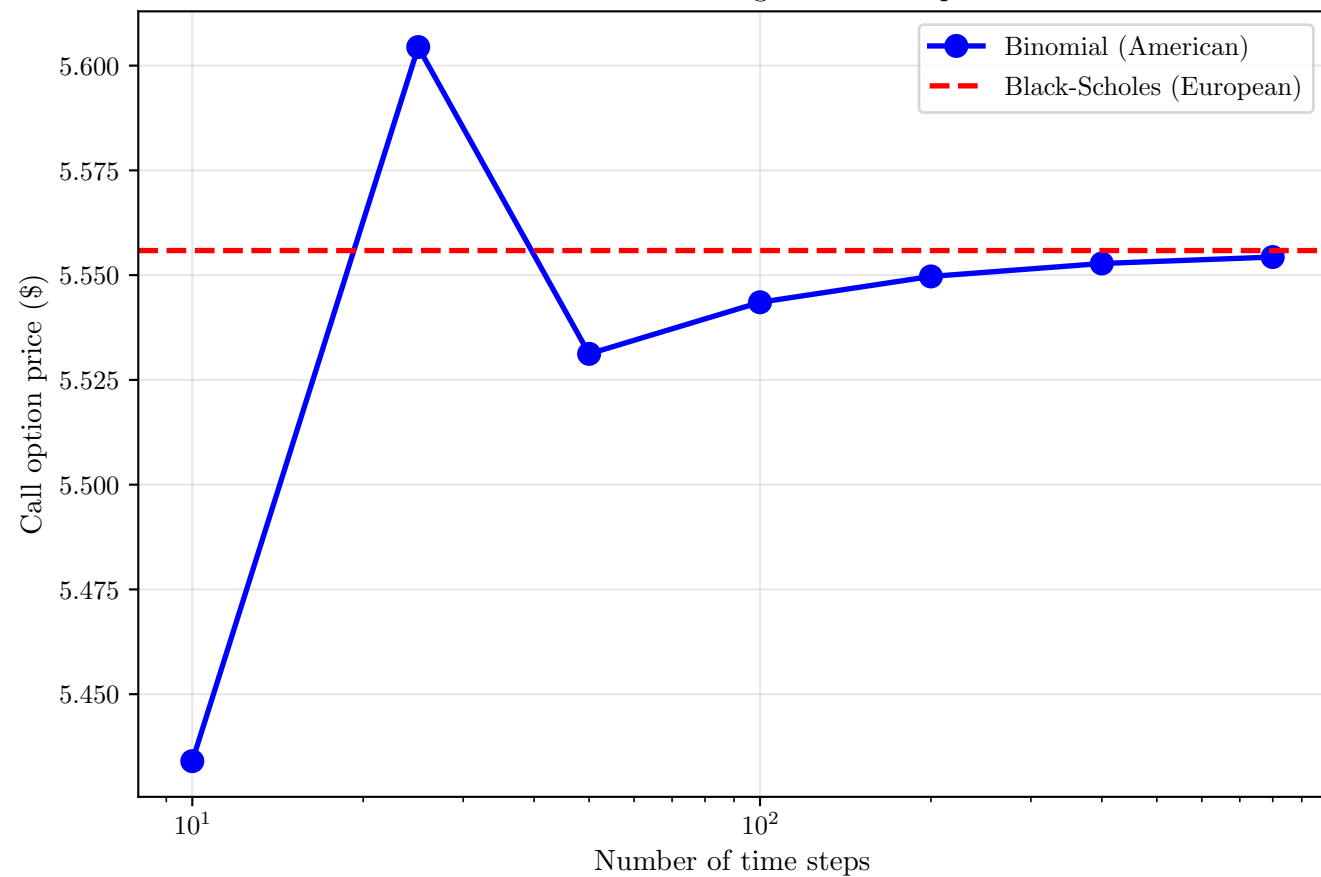
Binomial Tree Convergence: Call Option
