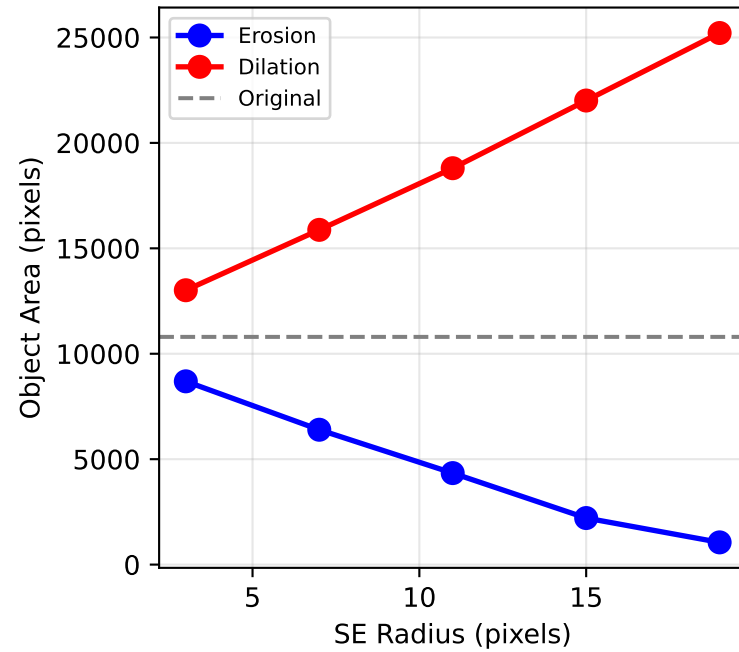
SE Size vs Object Area
