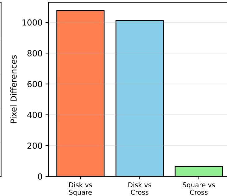
SE Shape Sensitivity
