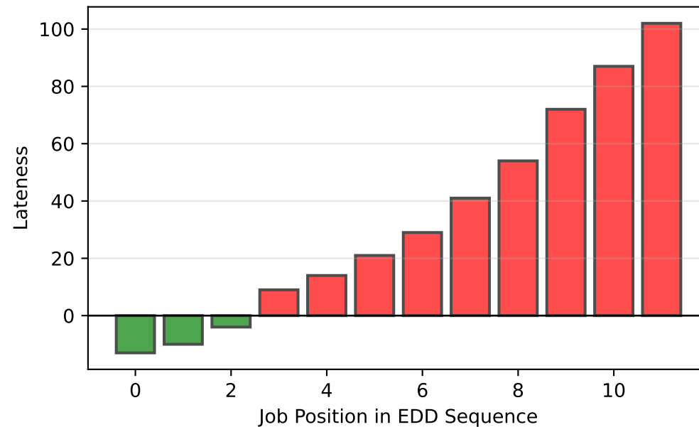
EDD Schedule: Lateness Profile (Max=102)
