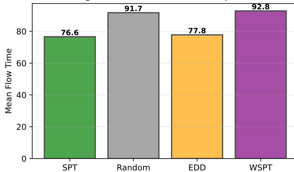
Single Machine: Flow Time Comparison
