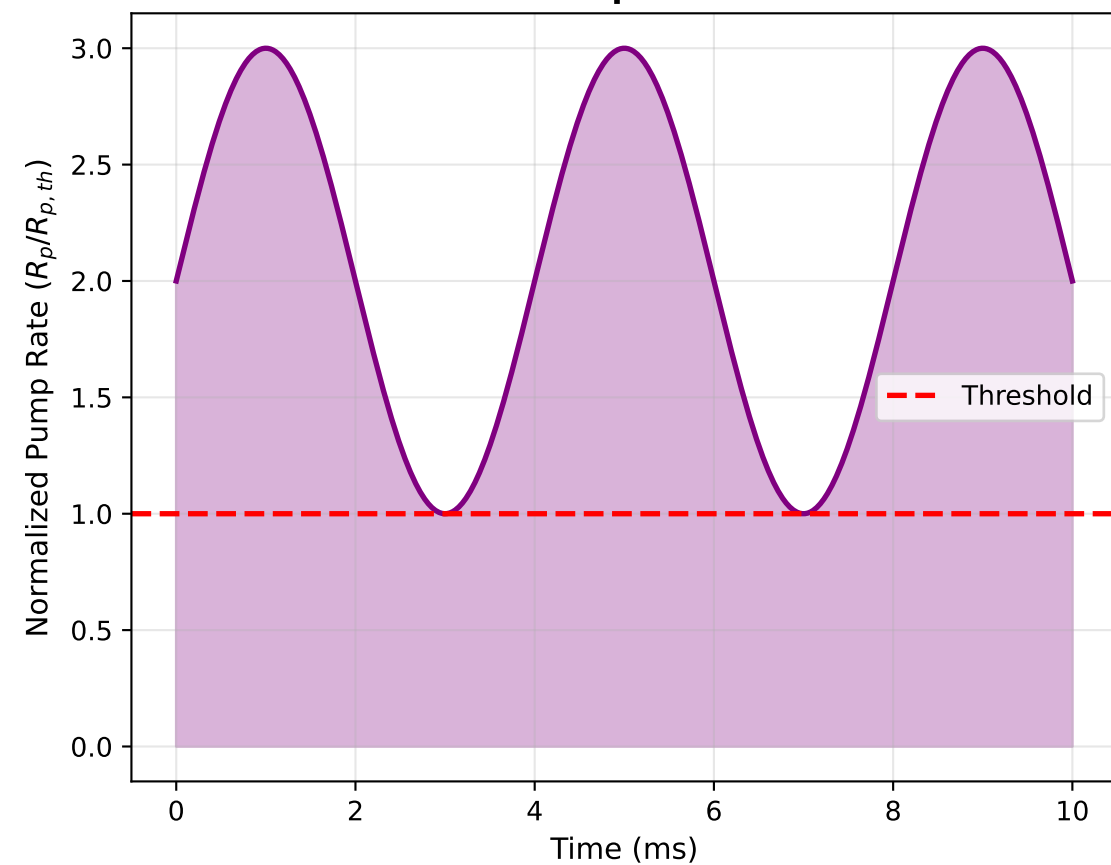
Pulsed Pump Modulation
