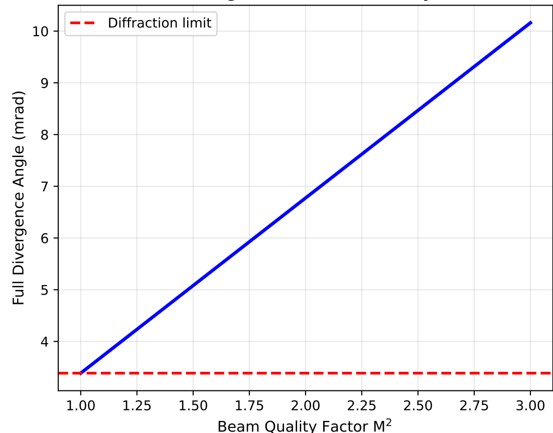
Divergence vs Beam Quality
