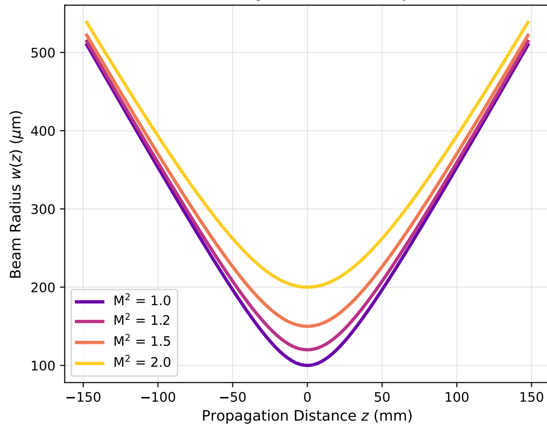
Beam Quality Factor M^2 Comparison
