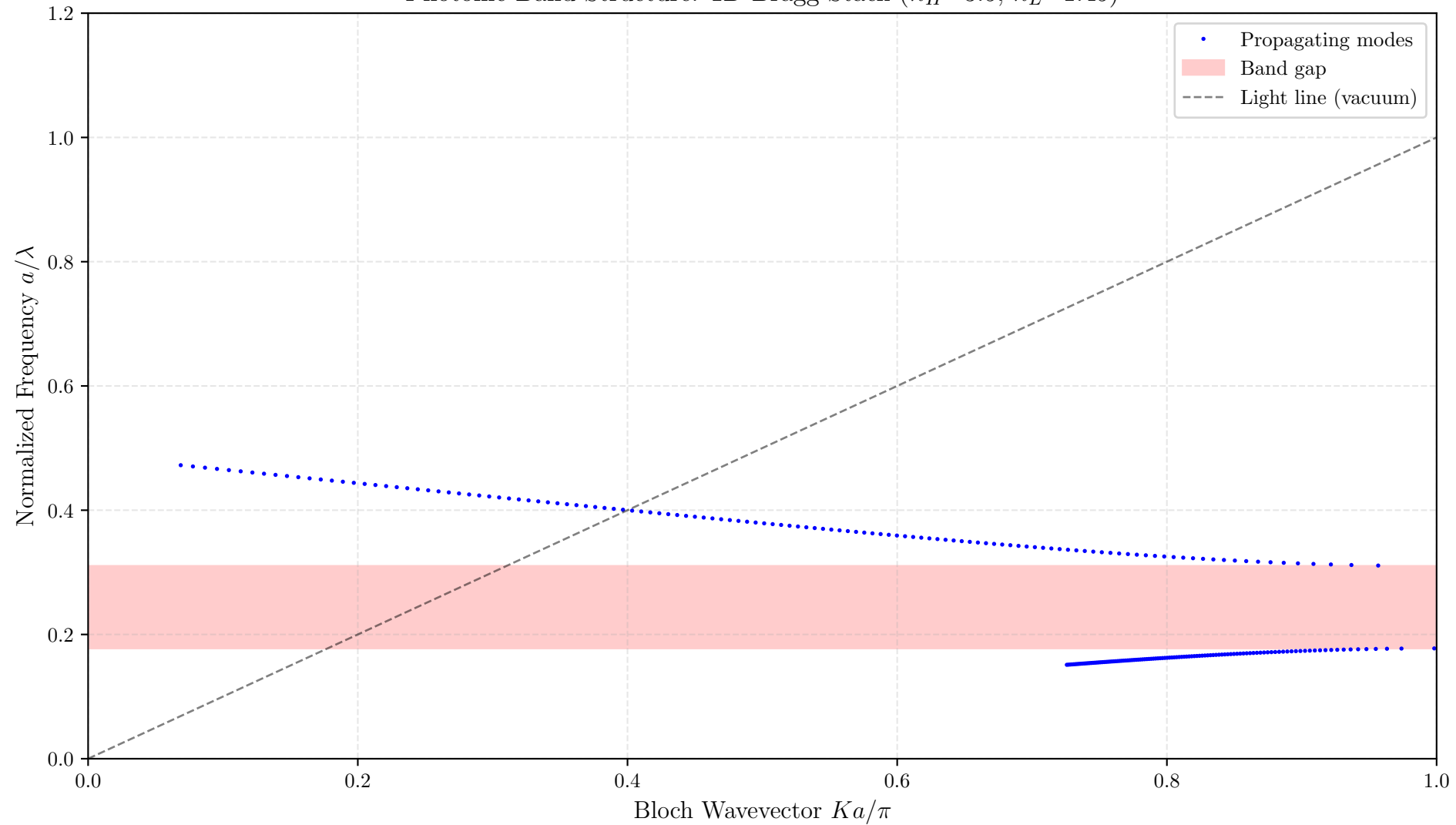
Photonic Band Structure: 1D Bragg Stack ( n_H=3.5 , n_L=1.45 )
