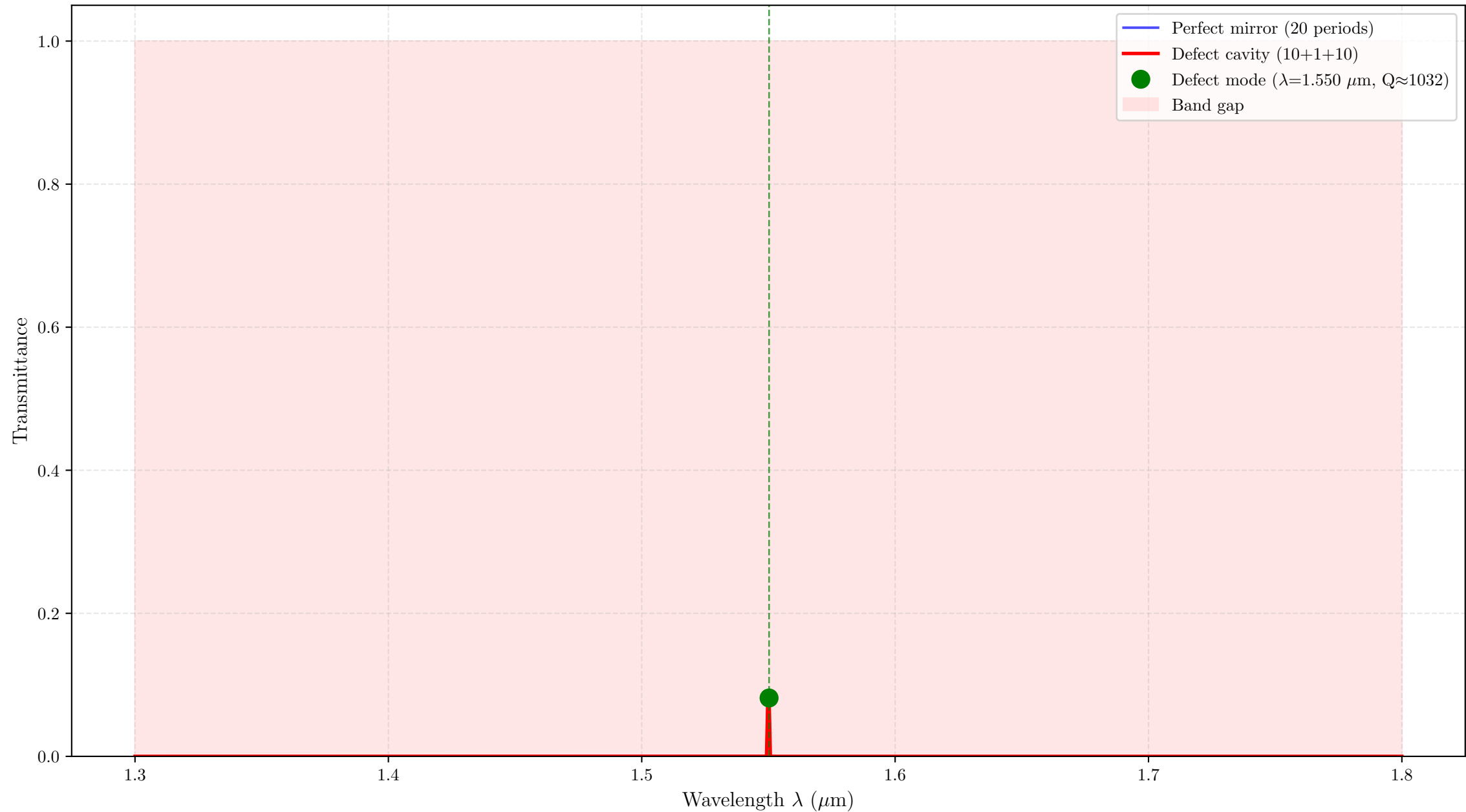
Defect Mode in 1D Photonic Crystal Cavity
