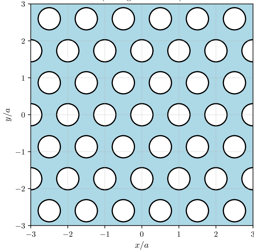
2D Photonic Crystal (Triangular Lattice)
