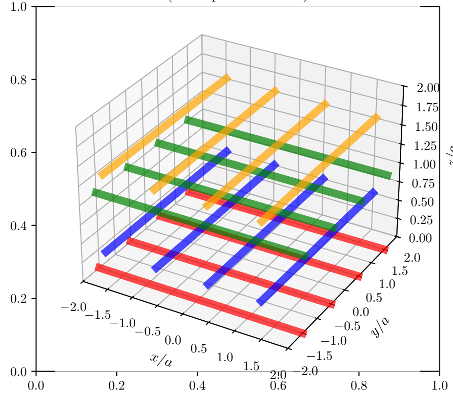
3D Photonic Crystal (Woodpile Structure)
