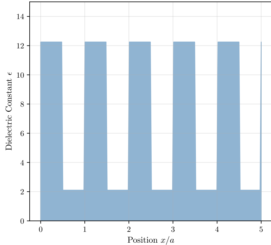
1D Photonic Crystal (Bragg Stack)
