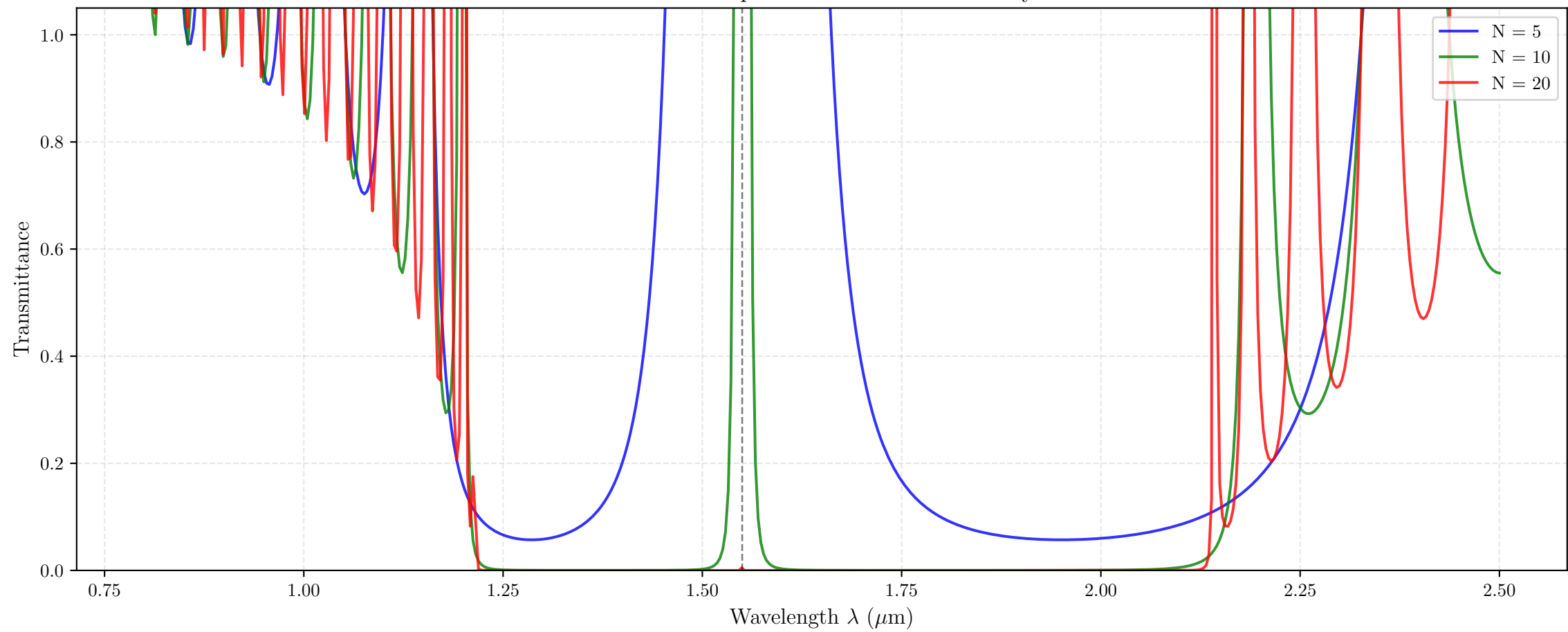
Transmittance Spectrum of 1D Photonic Crystal
