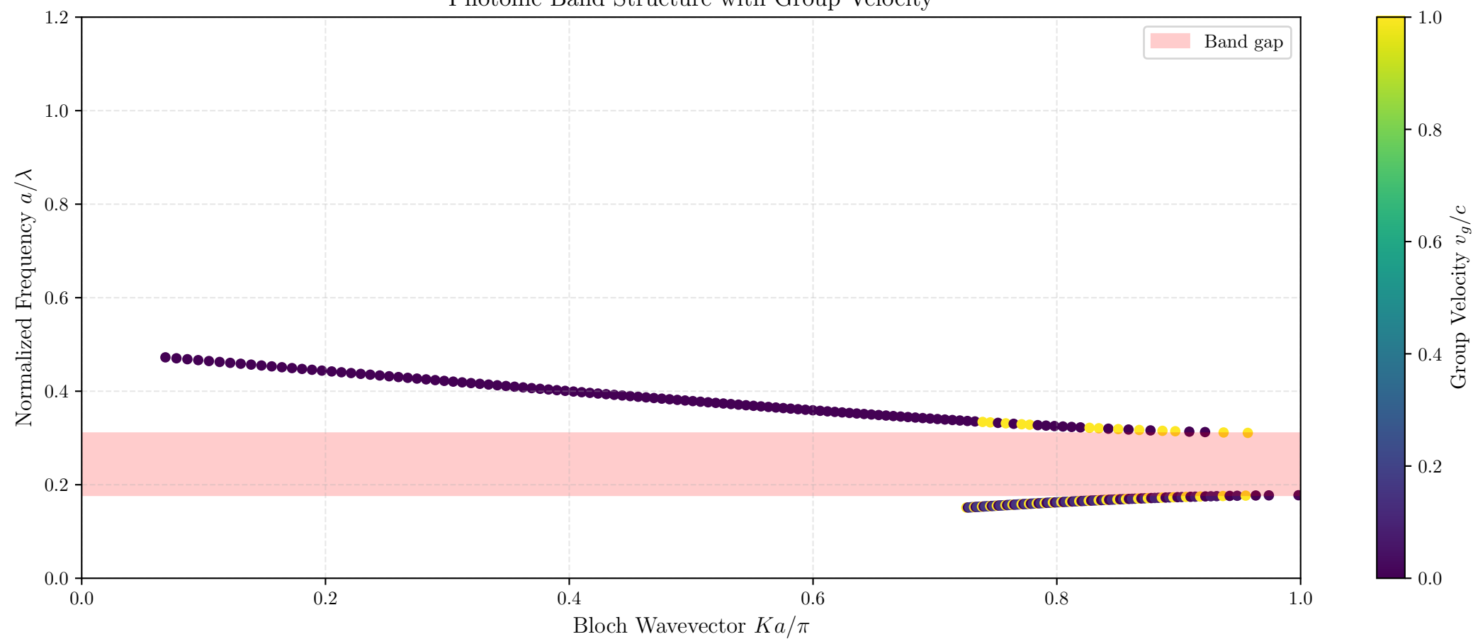
Group Velocity Dispersion
