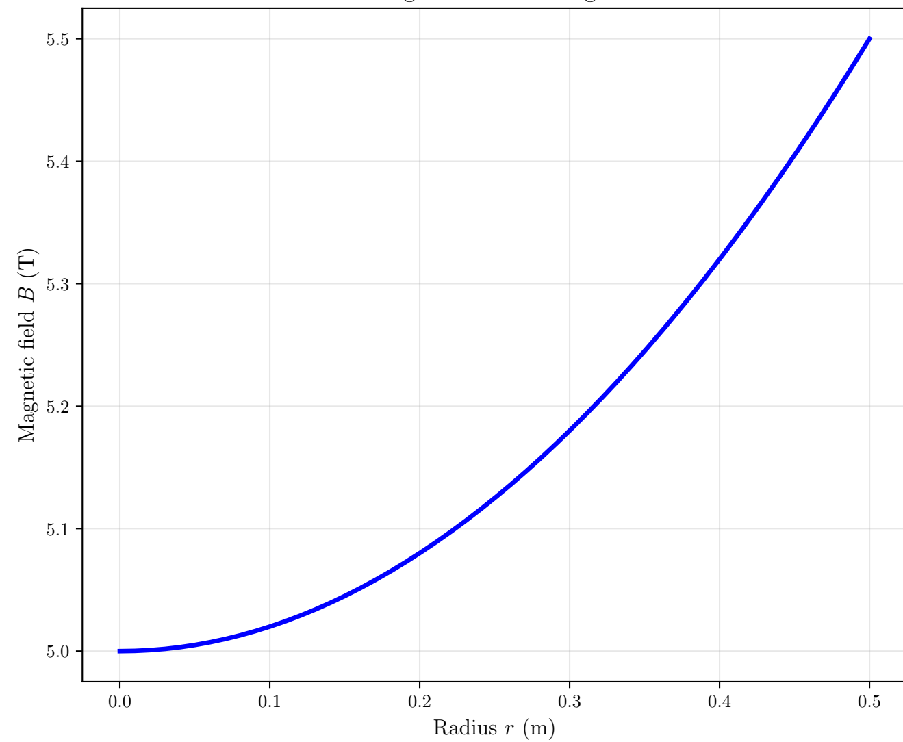
Magnetic Field Strength
