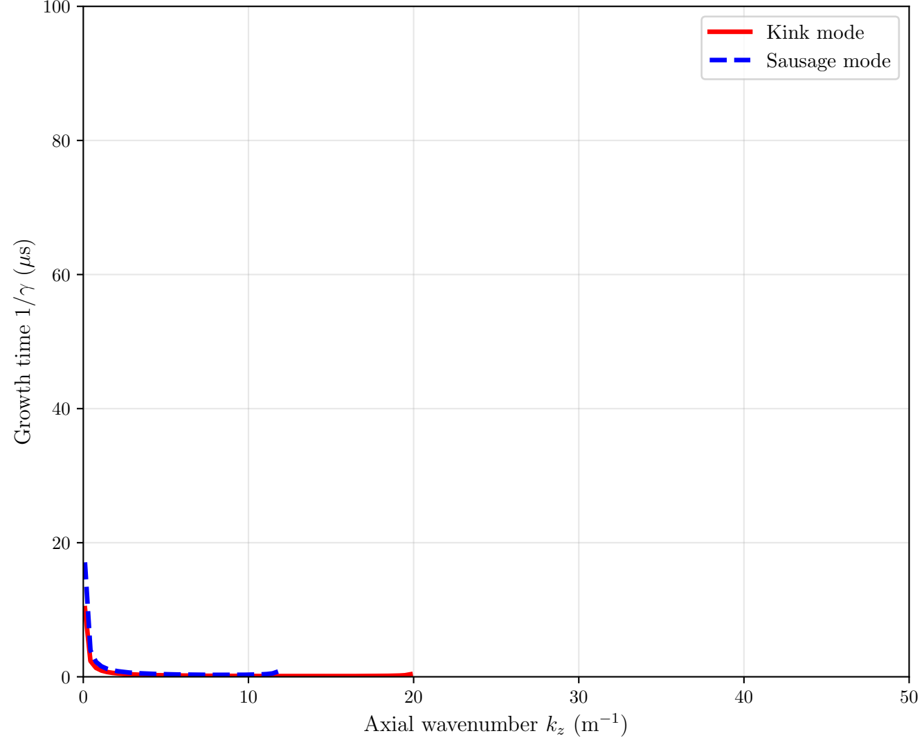
Instability Growth Timescales
