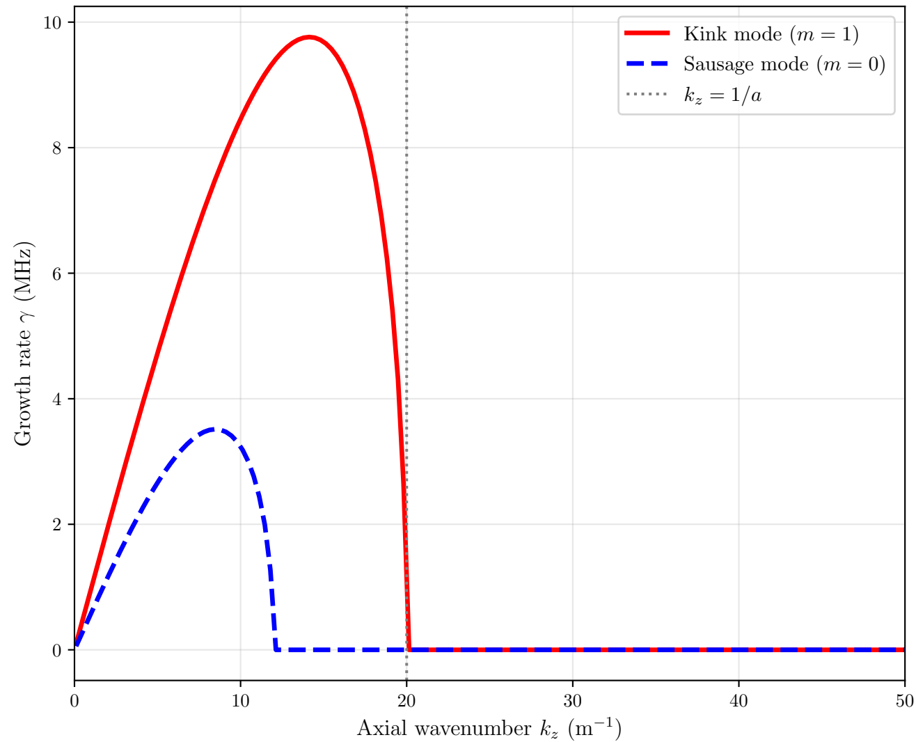
MHD Instability Growth Rates
