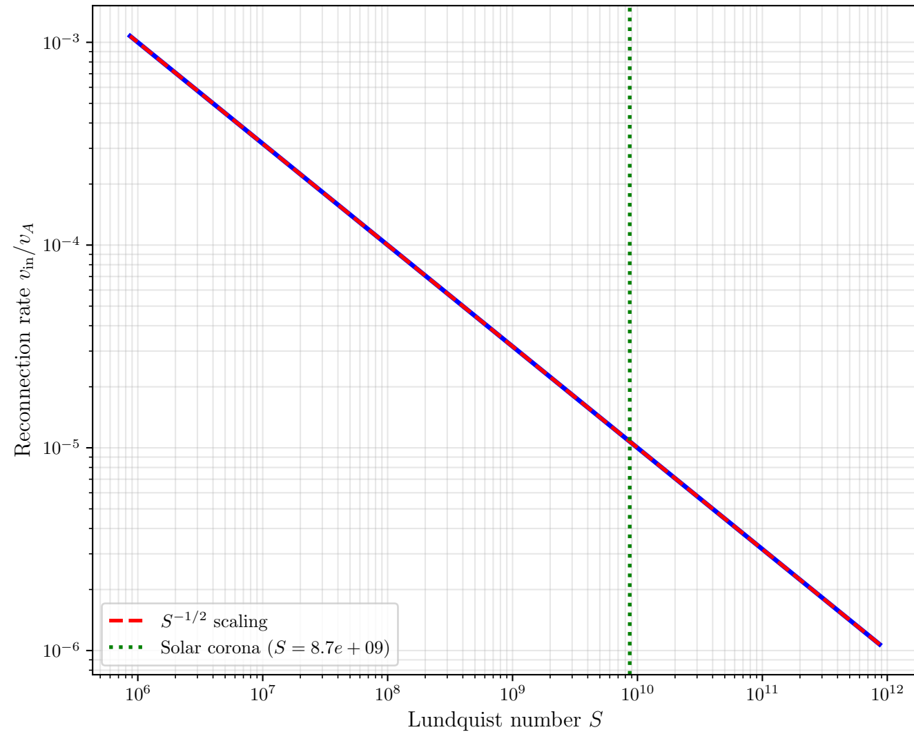
Sweet-Parker Reconnection Rate
