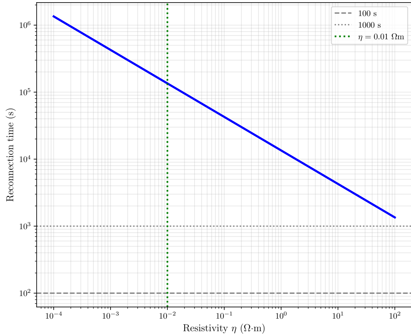
Reconnection Timescale vs Resistivity
