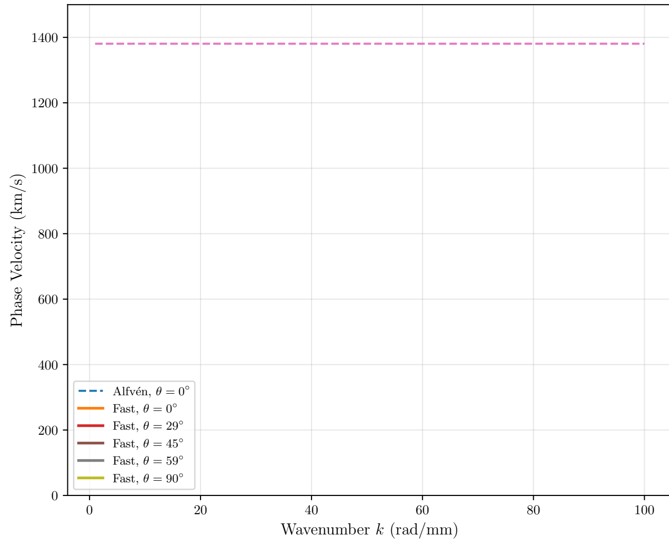
Fast Magnetosonic and Alfvén Modes
