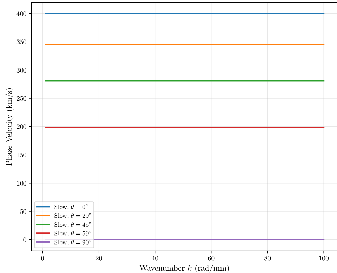
Slow Magnetosonic Mode
