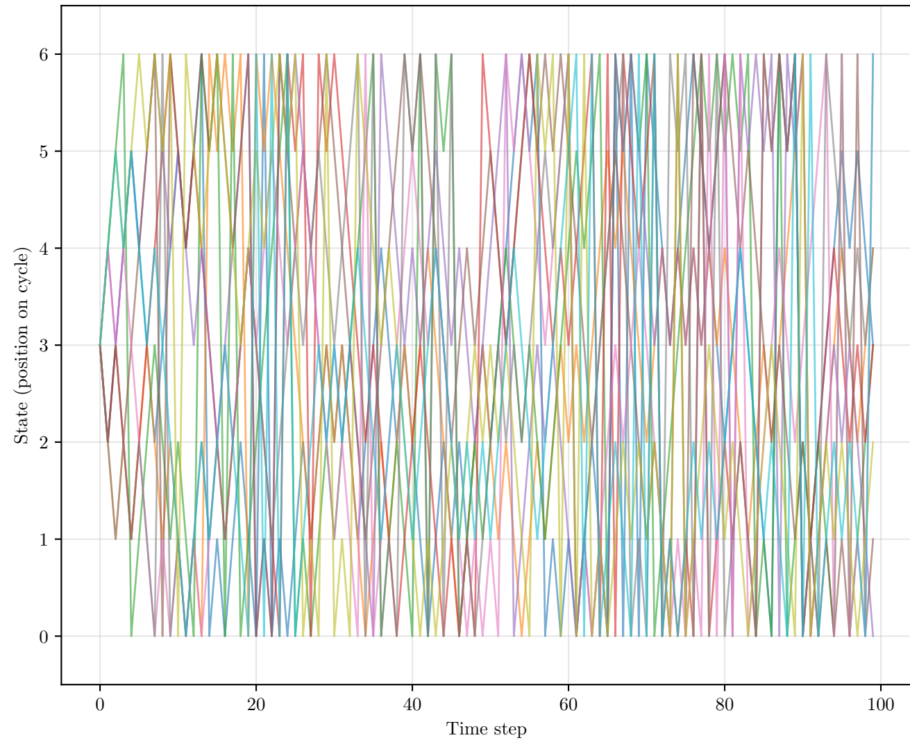
Symmetric Random Walk on Cycle Graph ( n = 7 )
