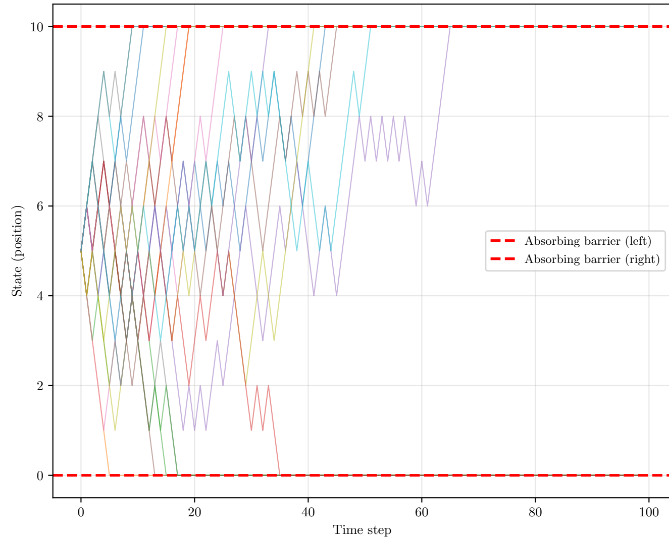
Random Walk with Absorbing Barriers
