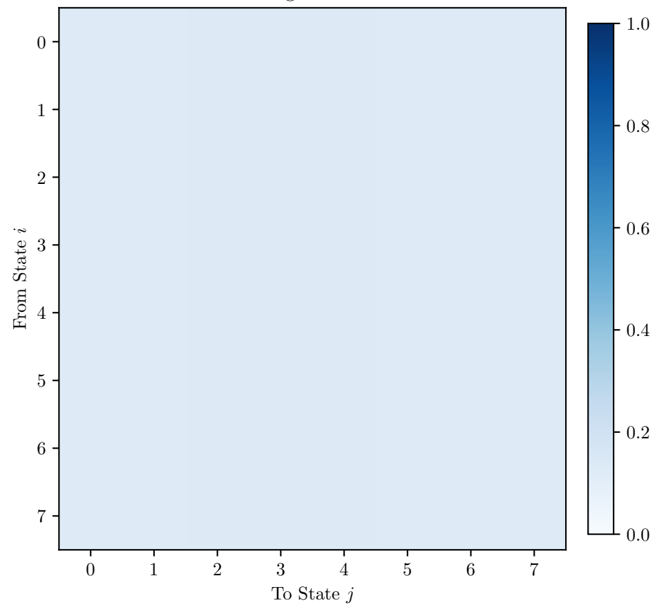
Limiting Matrix \mathbf{1}\pi^T
