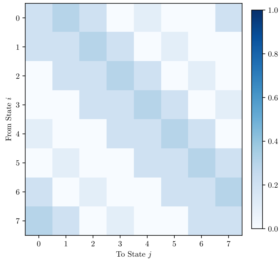
Transition Matrix P
