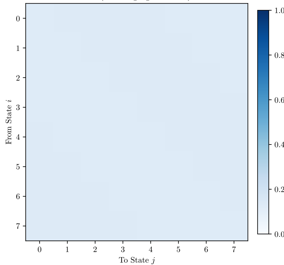
P^{50} (Converging to Limit)
