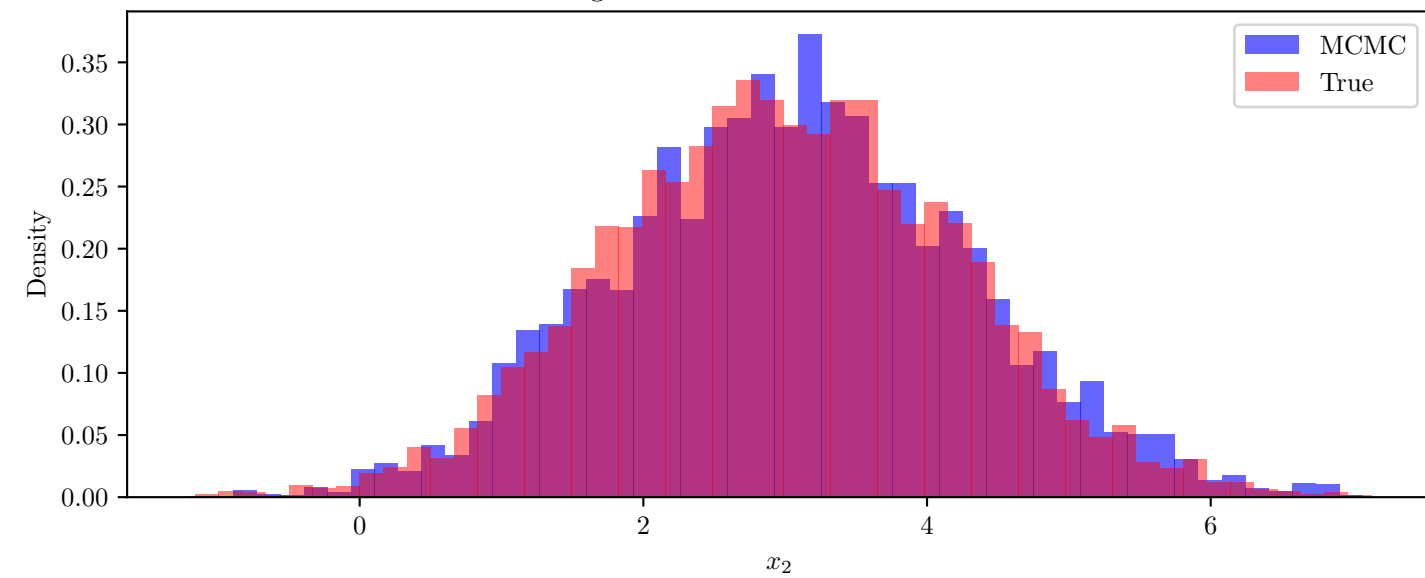
MCMC Sample Density (after burn-in)
