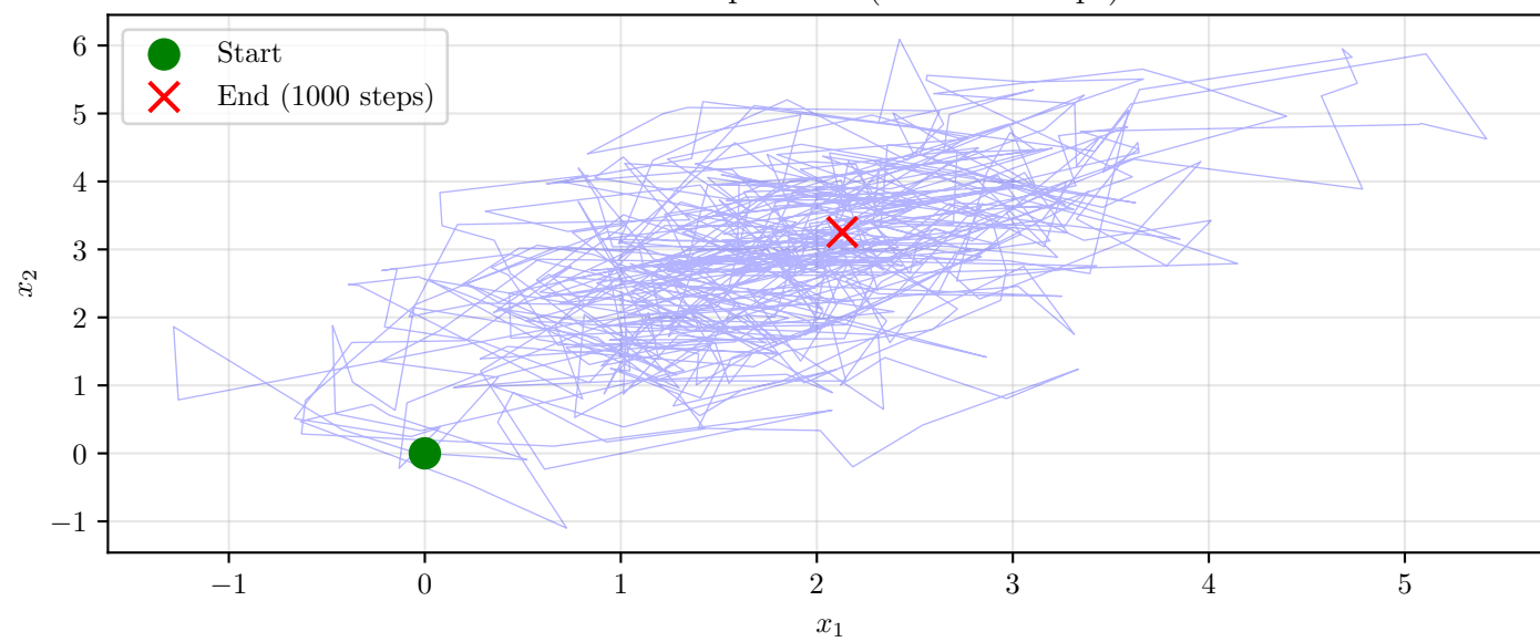
MCMC Sample Path (first 1000 steps)
