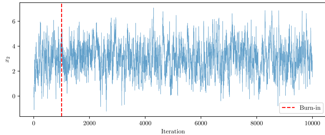
Marginal Distribution: Dimension 2
