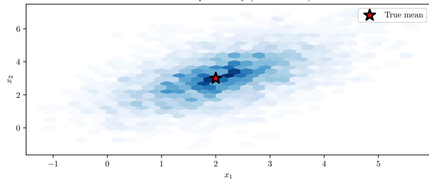
MCMC Sample Density (after burn-in)
