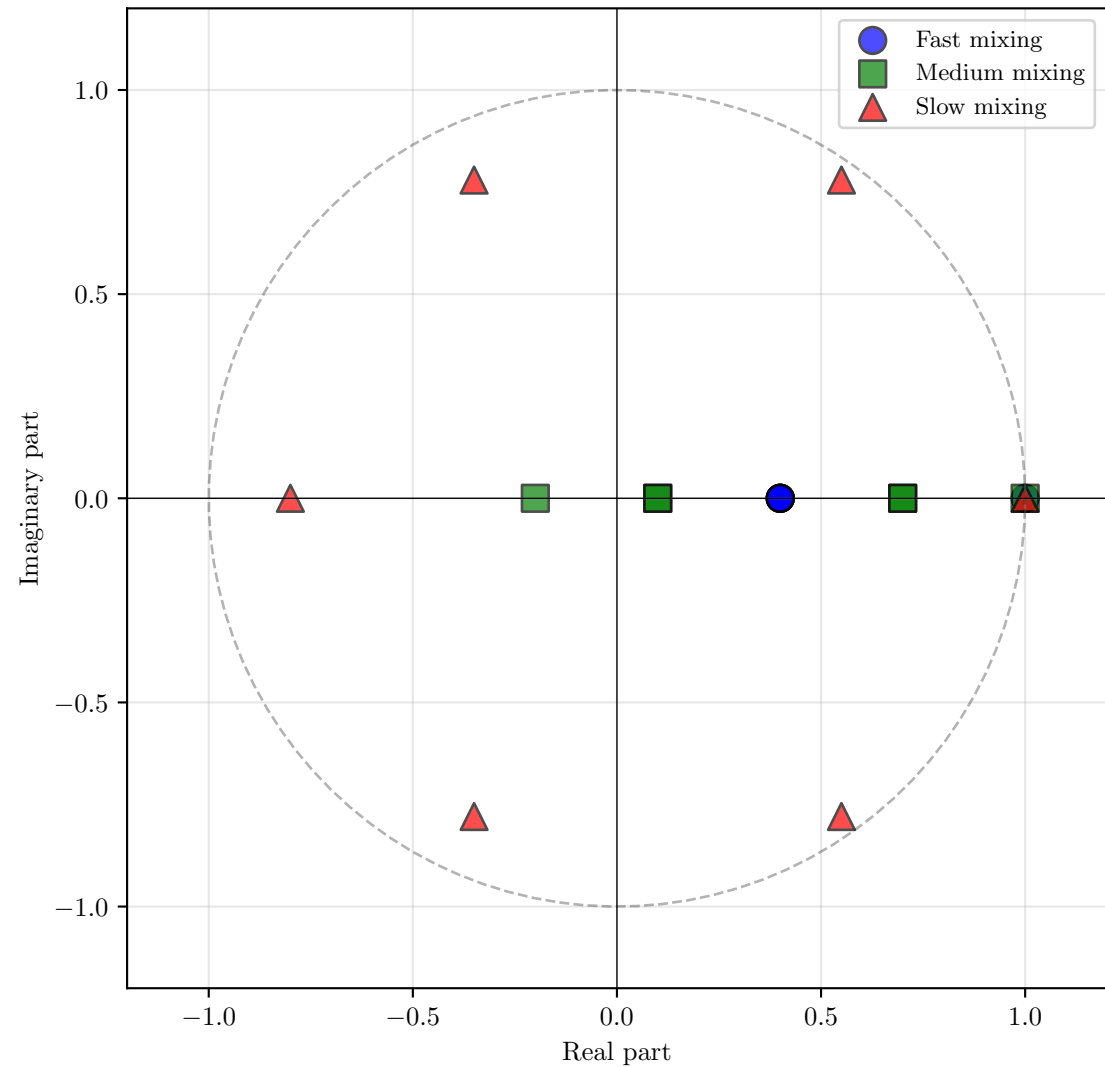
Eigenvalue Spectra in Complex Plane
