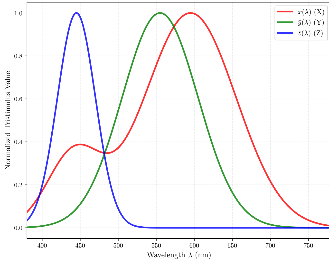
CIE 1931 Color Matching Functions
