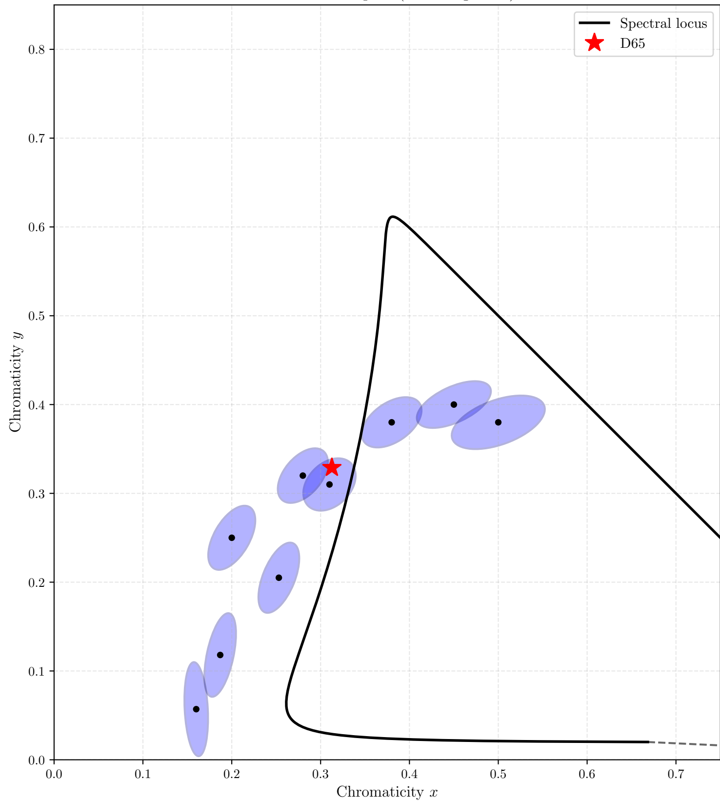
MacAdam Ellipses (10 \times magnified)
