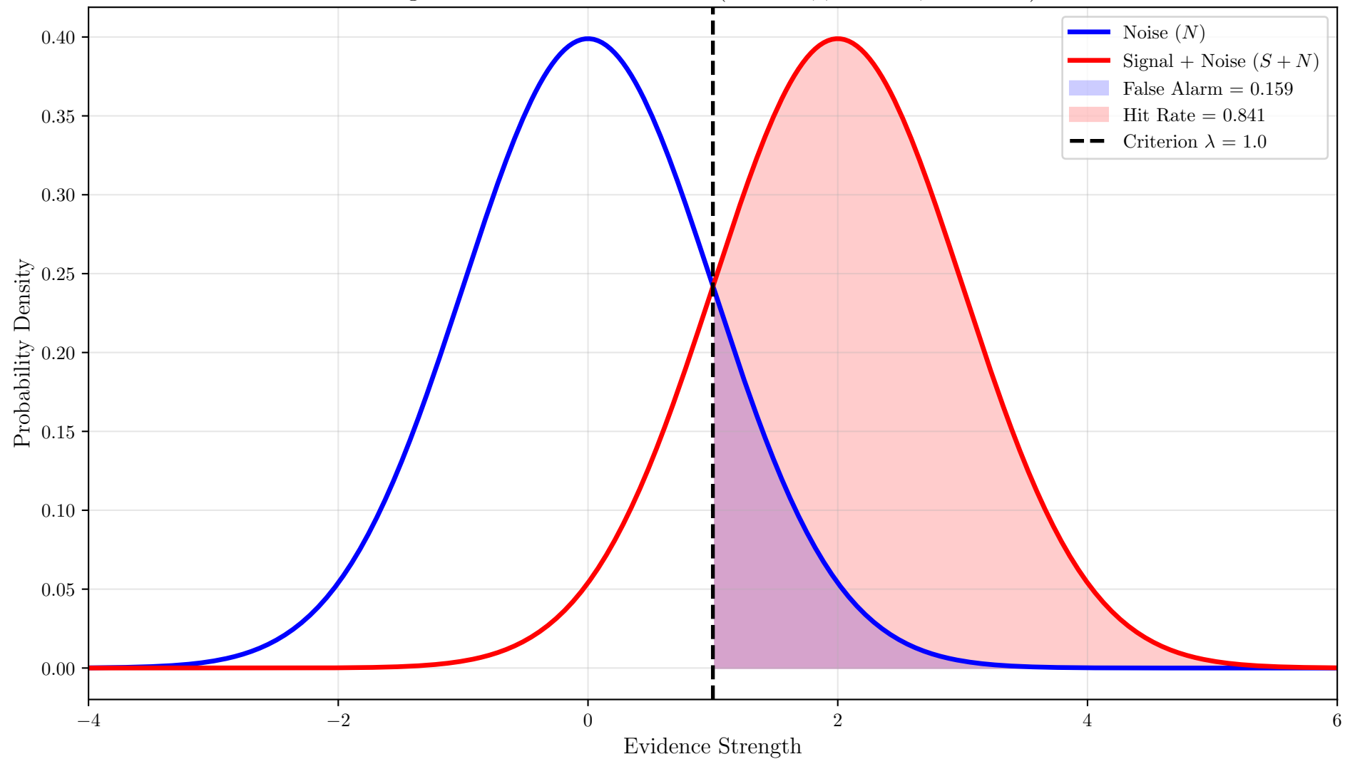
Signal and Noise Distributions ( d' = 2.0 , \beta = 1.00 , c = -0.00 )
