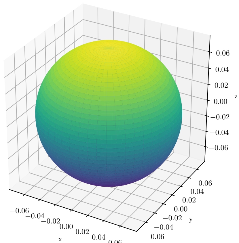
3d z^2 : Y_2^0
