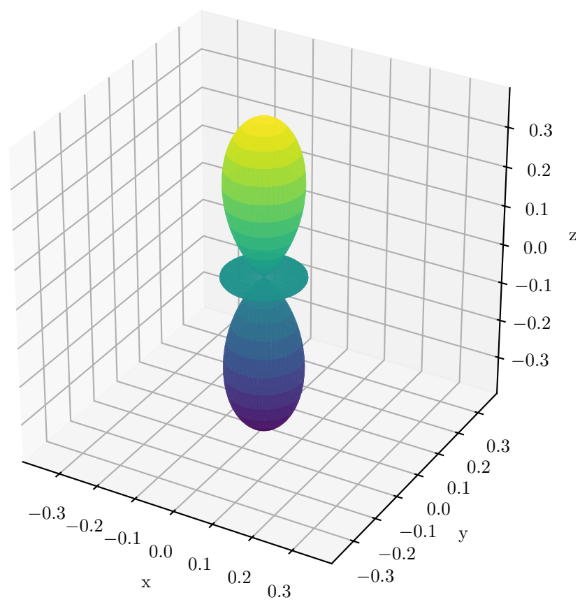
3d z^2 : Y_2^0
