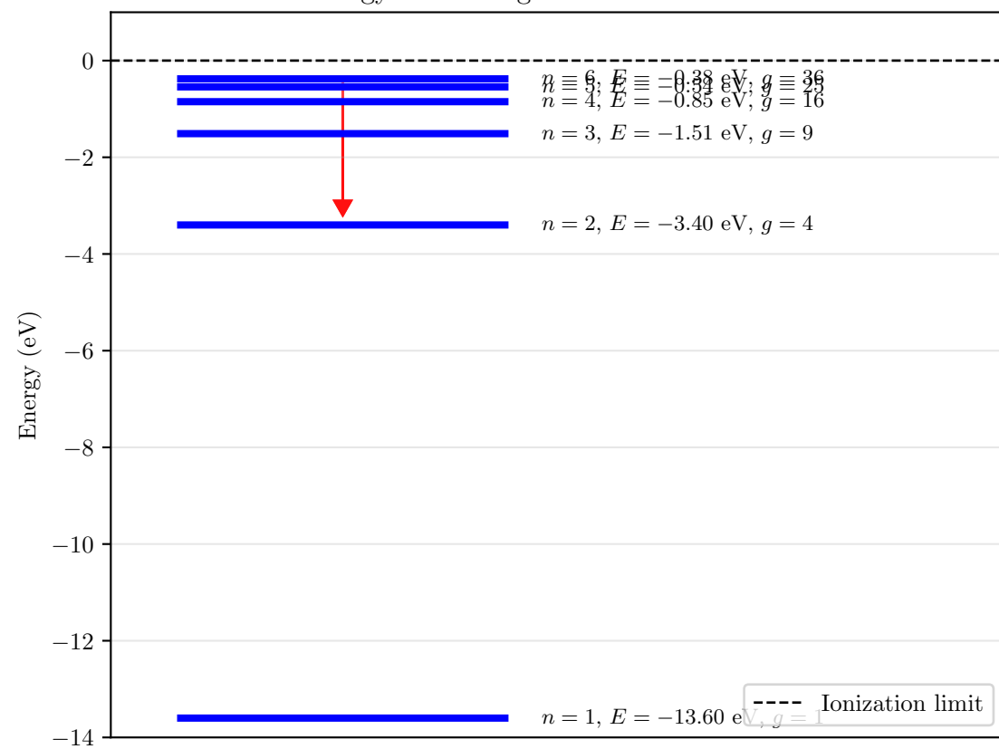
Energy Level Diagram and Balmer Series
