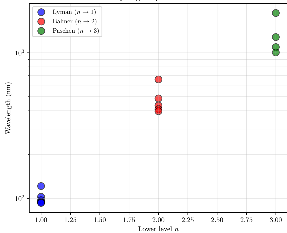
Hydrogen Spectral Series
