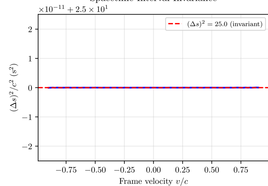
Spacetime Interval Invariance
