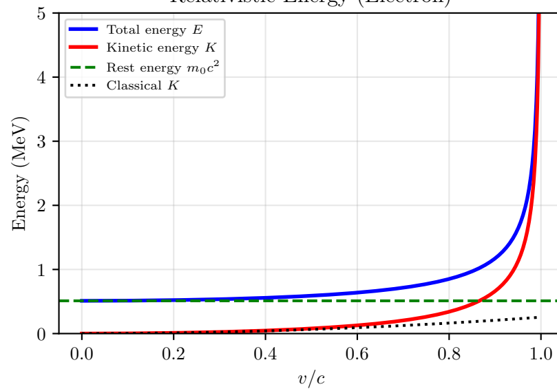
Relativistic Energy (Electron)
