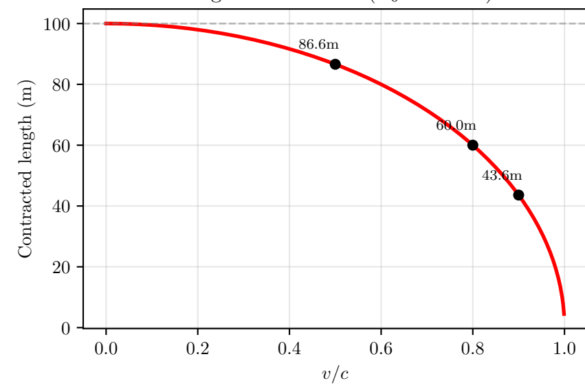
Length Contraction ( L_0 = 100 m)
