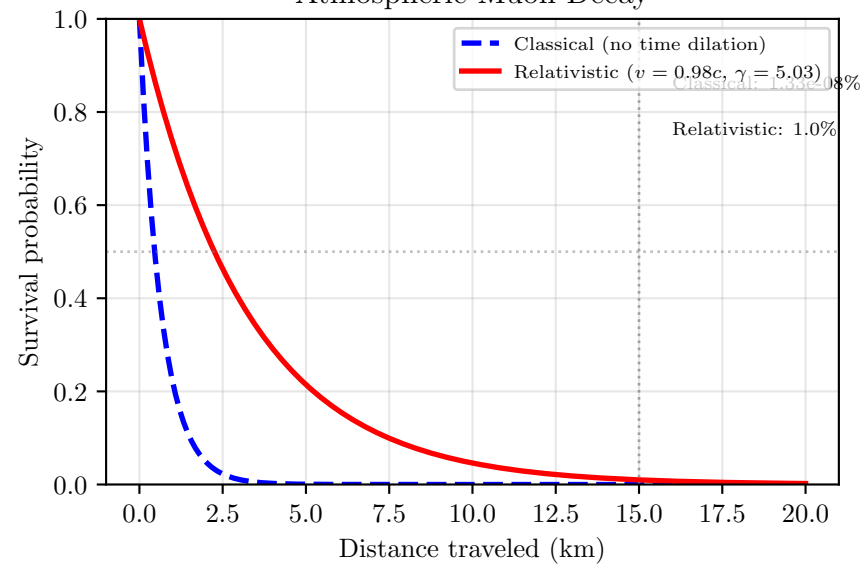
Atmospheric Muon Decay
