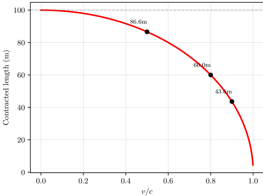
Length Contraction ( L_0 = 100\text{ m} )
