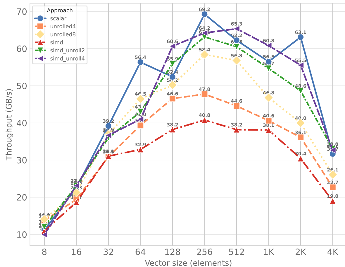
(a) Throughput by vector size
