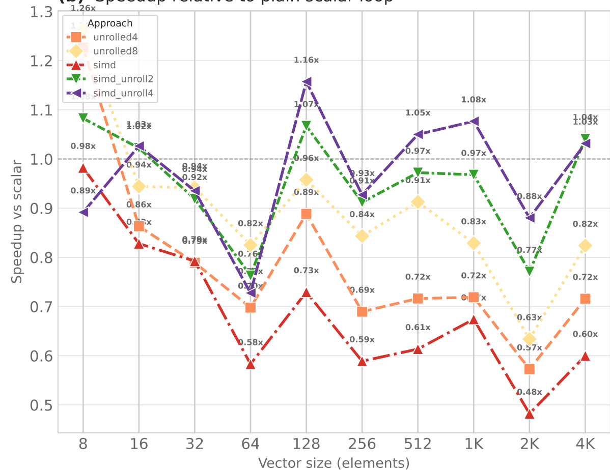
(b) Speedup relative to plain scalar loop
