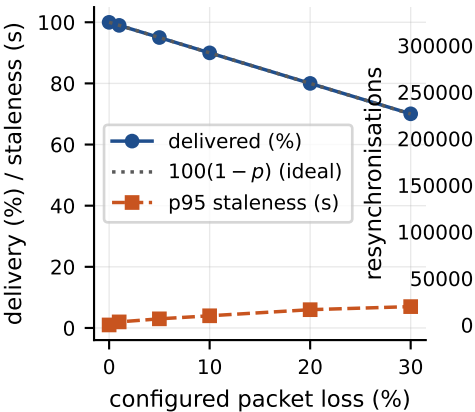
(a) loss sweep
