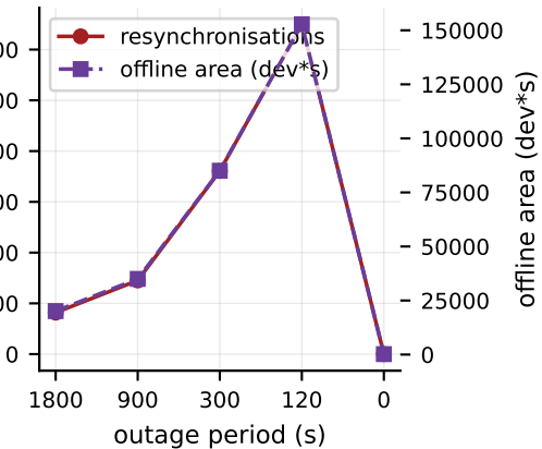
(b) outage frequency
