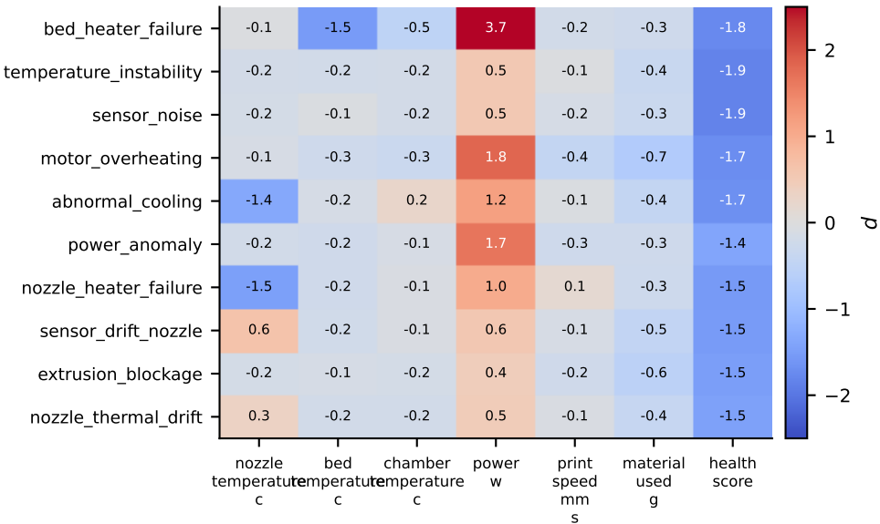
Cohen's d : faulted vs. healthy printing telemetry
