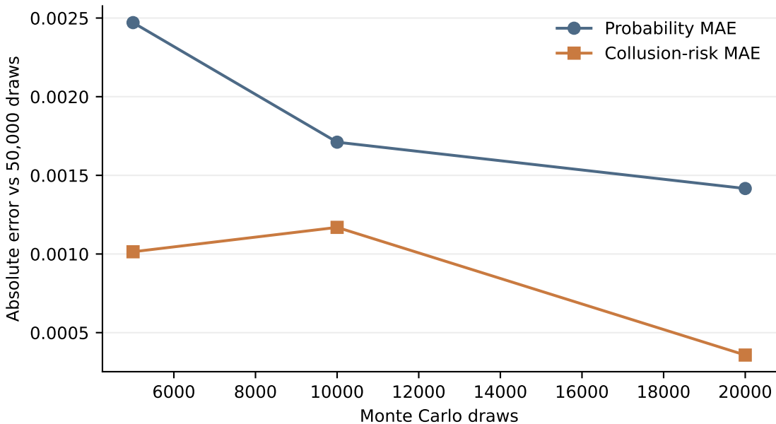
Q3 simulation convergence
