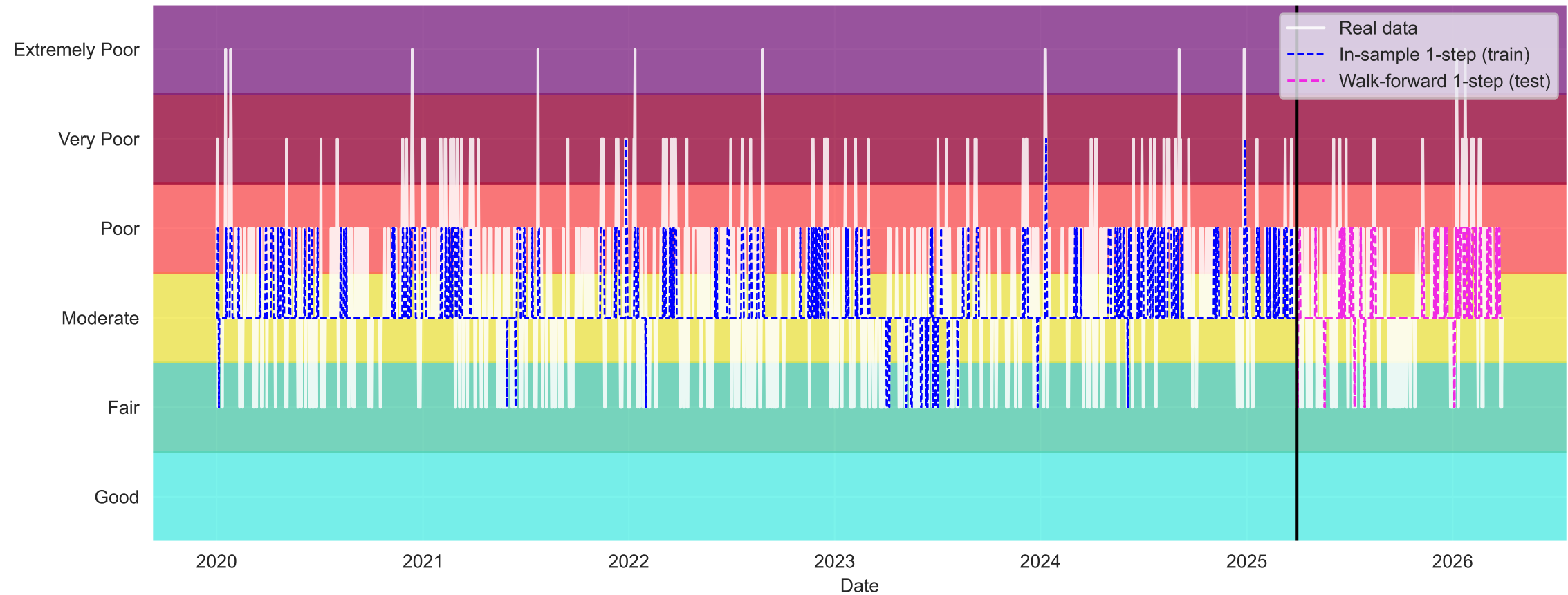
EAQI Daily Air Quality Index — ARIMAX (dummies)
