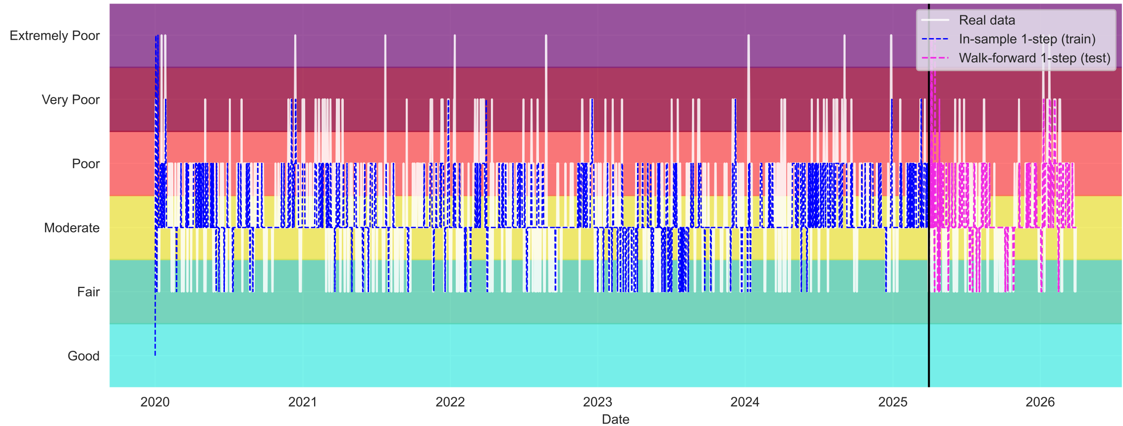
EAQI Daily Air Quality Index — SARIMA (meteo)
