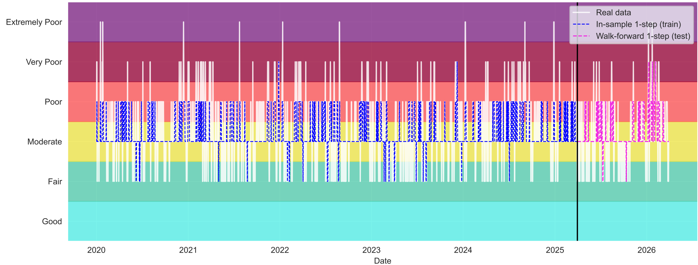
EAQI Daily Air Quality Index — VARX (dummies + meteo)
