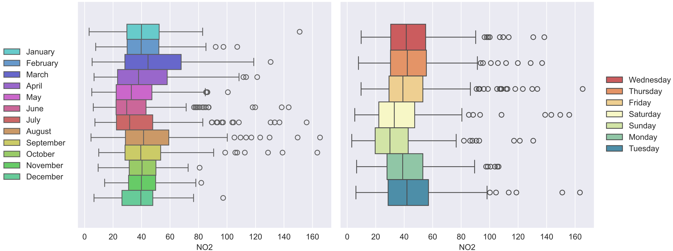
Boxplots of NO2 by Month and by Weekday
