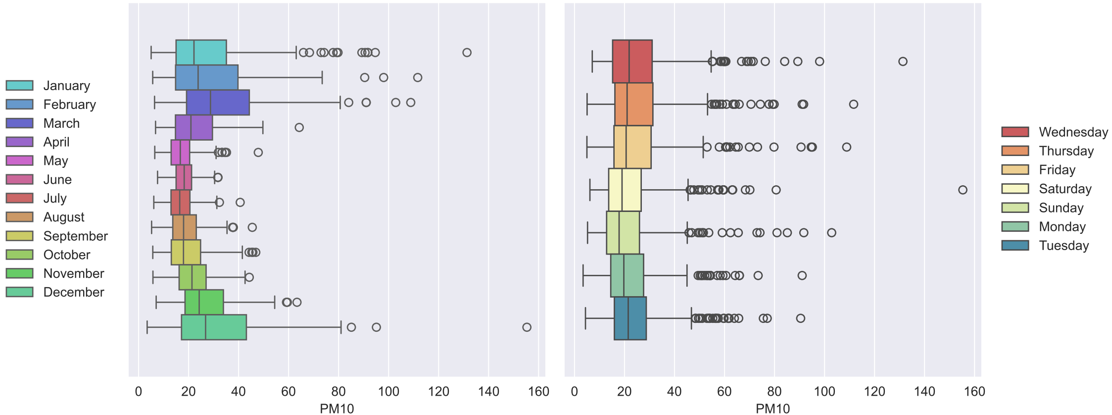
Boxplots of PM10 by Month and by Weekday
